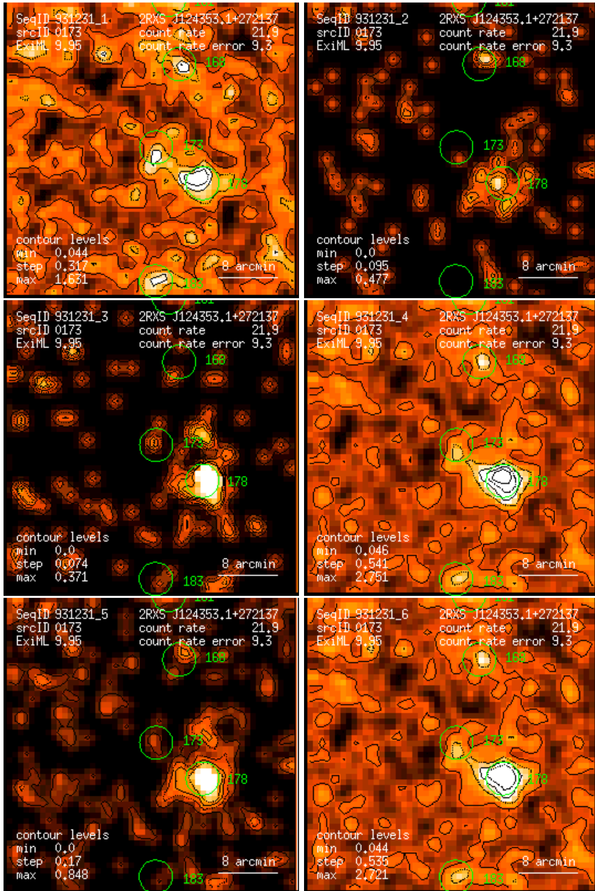
Figure 173: RASS 931231: detection 0173: band rate images, Gaussian filter: (1) PSPC channels 11 – 41, (2) 52 – 90, (3) 91 – 201, (4) 11 – 235, (5) 52 – 201, (6) 11 – 201. Broad band rates in counts/ks. Band rate contour levels in counts/ks/arcmin 2 .
