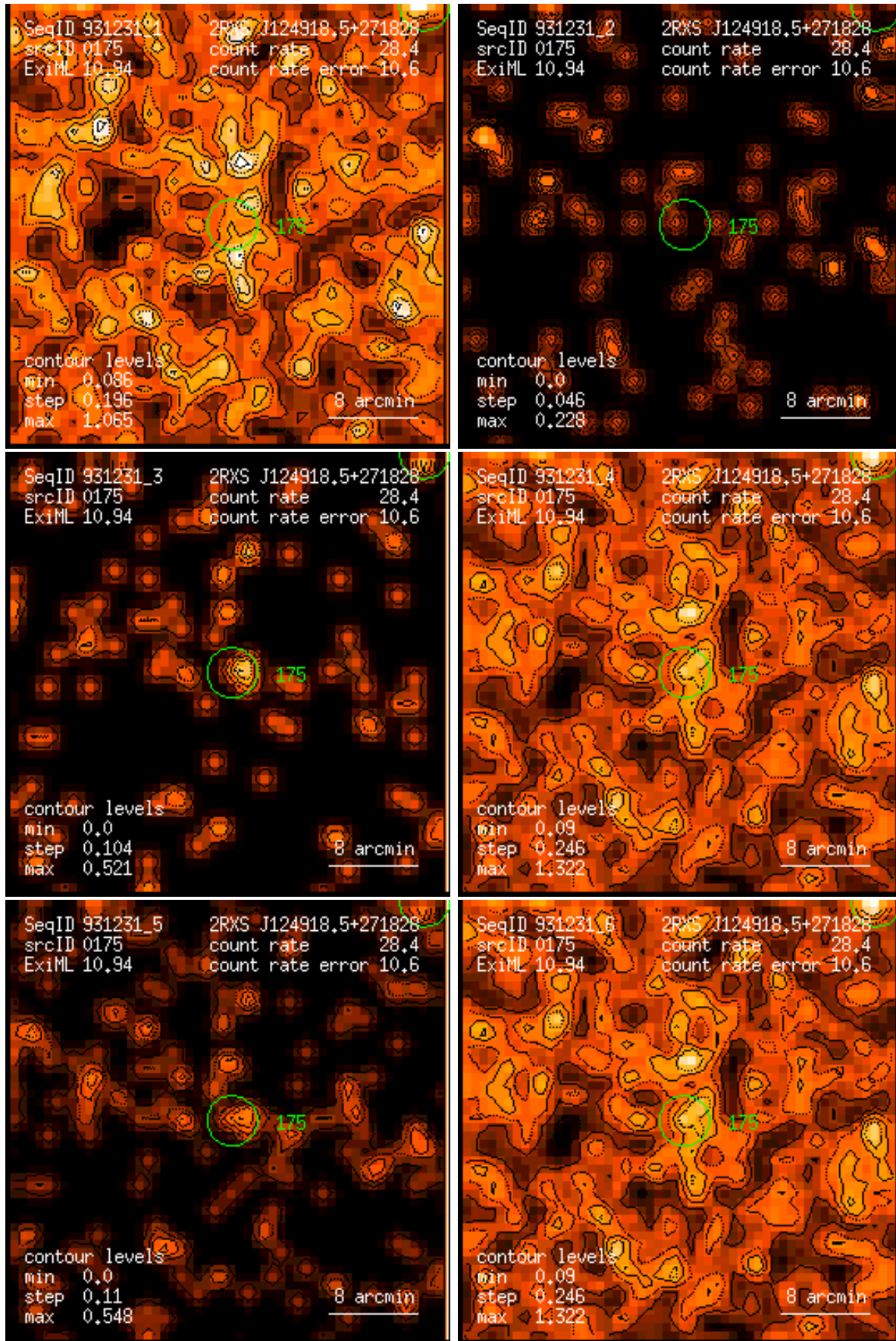
Figure 175: RASS 931231: detection 0175: band rate images, Gaussian filter: (1) PSPC channels 11 – 41, (2) 52 – 90, (3) 91 – 201, (4) 11 – 235, (5) 52 – 201, (6) 11 – 201. Broad band rates in counts/ks. Band rate contour levels in counts/ks/arcmin 2 .
