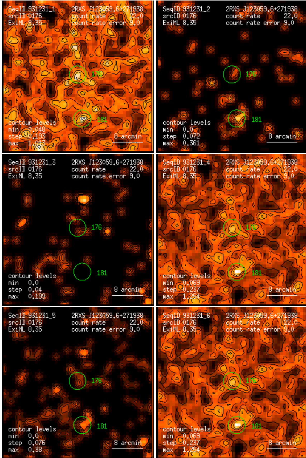
Figure 176: RASS 931231: detection 0176: band rate images, Gaussian filter: (1) PSPC channels 11 – 41, (2) 52 – 90, (3) 91 – 201, (4) 11 – 235, (5) 52 – 201, (6) 11 – 201. Broad band rates in counts/ks. Band rate contour levels in counts/ks/arcmin 2 .
