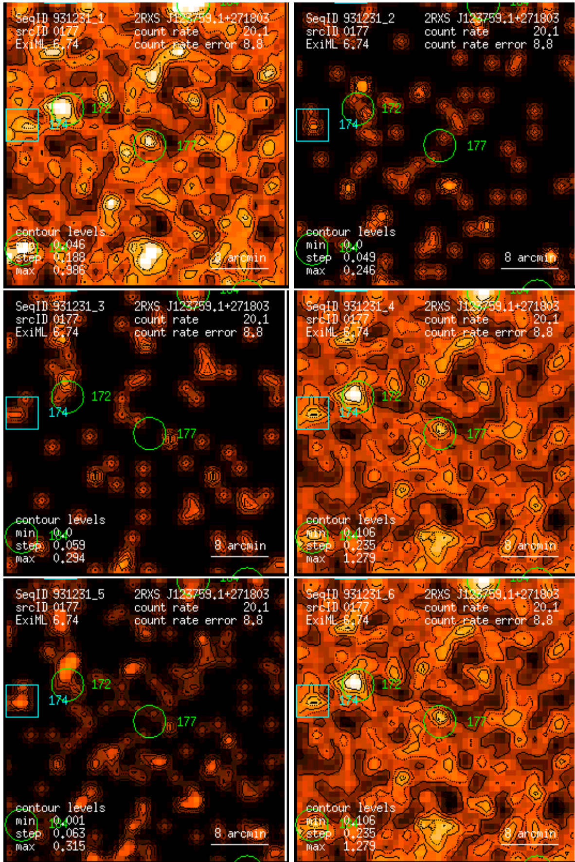
Figure 177: RASS 931231: detection 0177: band rate images, Gaussian filter: (1) PSPC channels 11 – 41, (2) 52 – 90, (3) 91 – 201, (4) 11 – 235, (5) 52 – 201, (6) 11 – 201. Broad band rates in counts/ks. Band rate contour levels in counts/ks/arcmin 2 .
