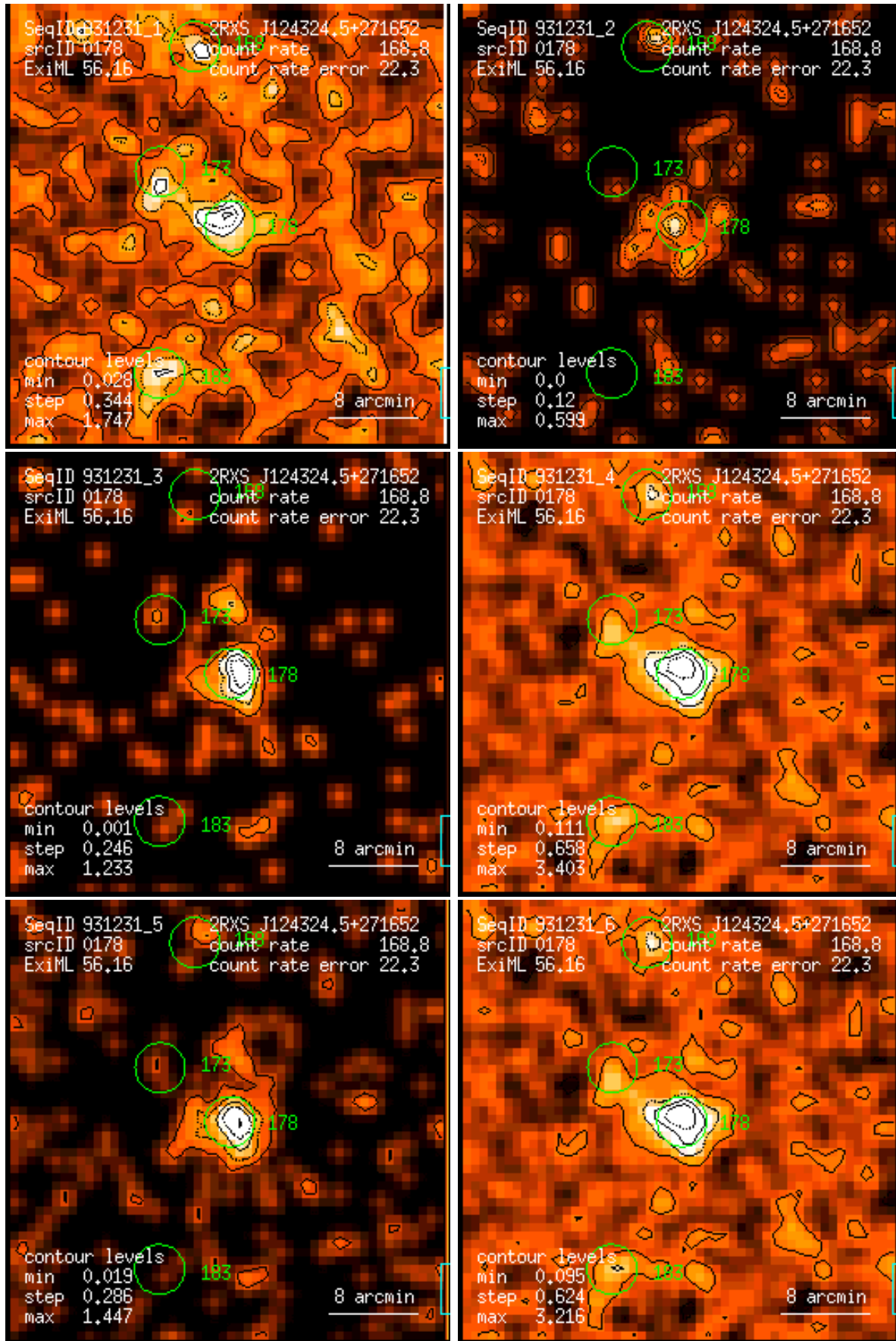
Figure 178: RASS 931231: detection 0178: band rate images, Gaussian filter: (1) PSPC channels 11 – 41, (2) 52 – 90, (3) 91 – 201, (4) 11 – 235, (5) 52 – 201, (6) 11 – 201. Broad band rates in counts/ks. Band rate contour levels in counts/ks/arcmin 2 .
