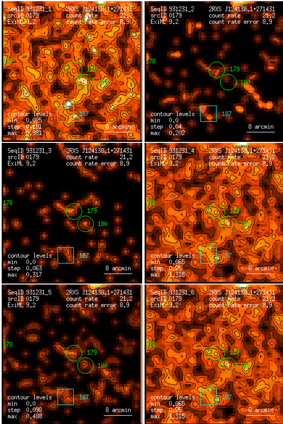
Figure 179: RASS 931231: detection 0179: band rate images, Gaussian filter: (1) PSPC channels 11 – 41, (2) 52 – 90, (3) 91 – 201, (4) 11 – 235, (5) 52 – 201, (6) 11 – 201. Broad band rates in counts/ks. Band rate contour levels in counts/ks/arcmin 2 .
