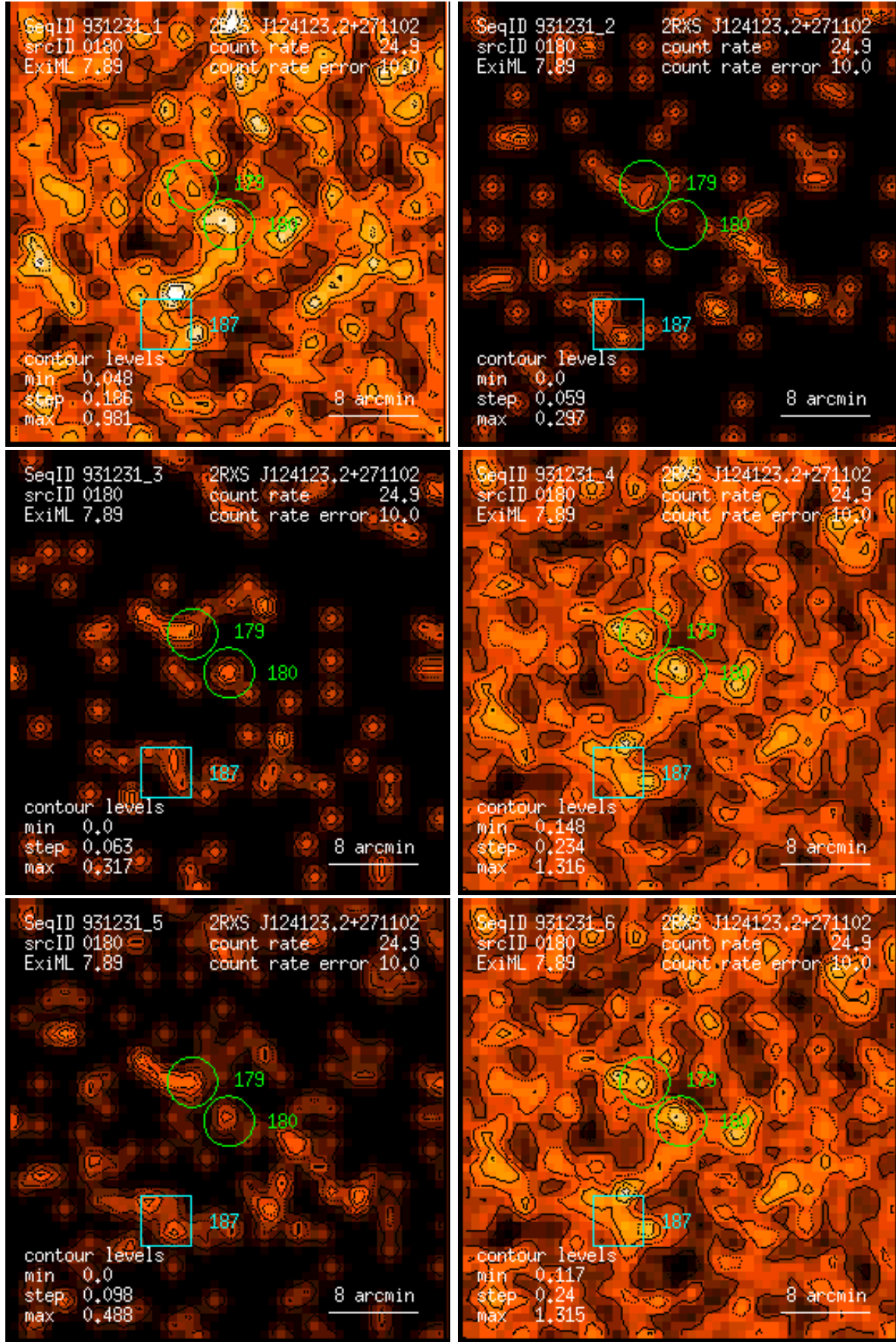
Figure 180: RASS 931231: detection 0180: band rate images, Gaussian filter: (1) PSPC channels 11 – 41, (2) 52 – 90, (3) 91 – 201, (4) 11 – 235, (5) 52 – 201, (6) 11 – 201. Broad band rates in counts/ks. Band rate contour levels in counts/ks/arcmin 2 .
