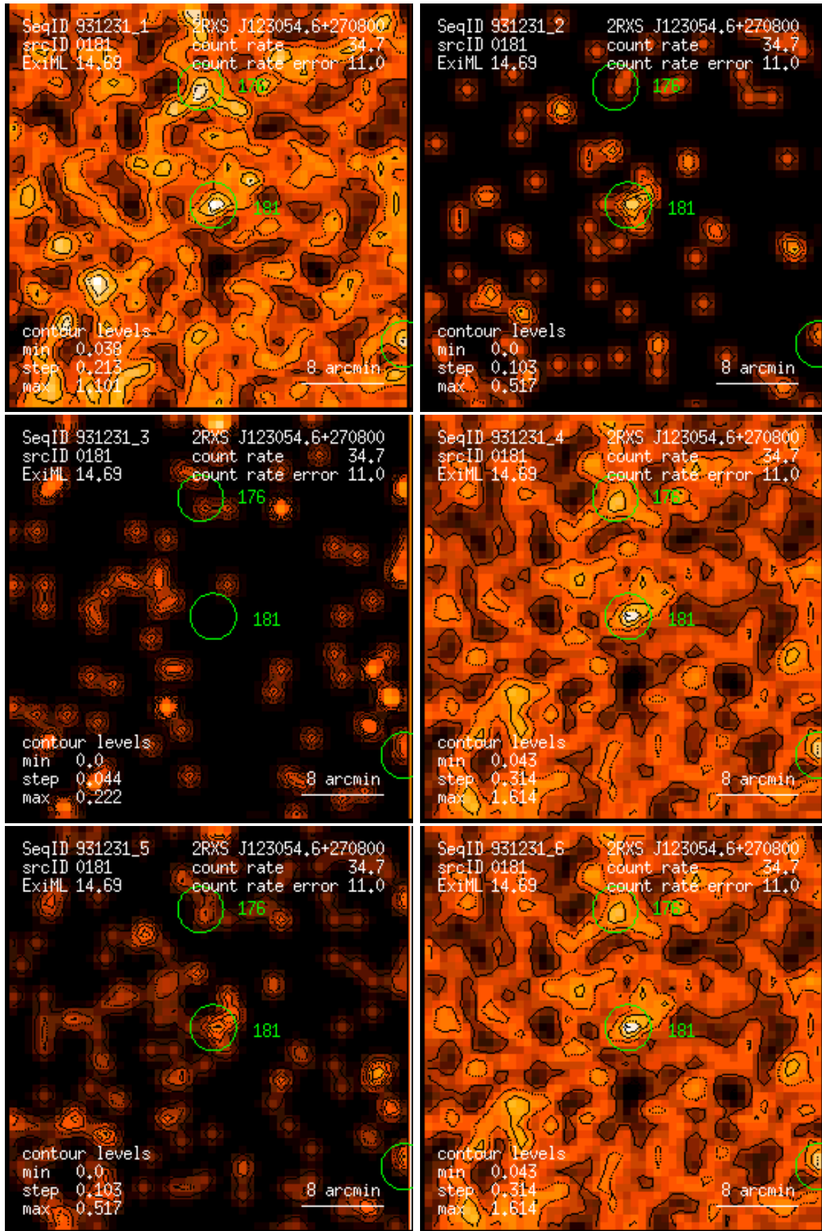
Figure 181: RASS 931231: detection 0181: band rate images, Gaussian filter: (1) PSPC channels 11 – 41, (2) 52 – 90, (3) 91 – 201, (4) 11 – 235, (5) 52 – 201, (6) 11 – 201. Broad band rates in counts/ks. Band rate contour levels in counts/ks/arcmin 2 .
