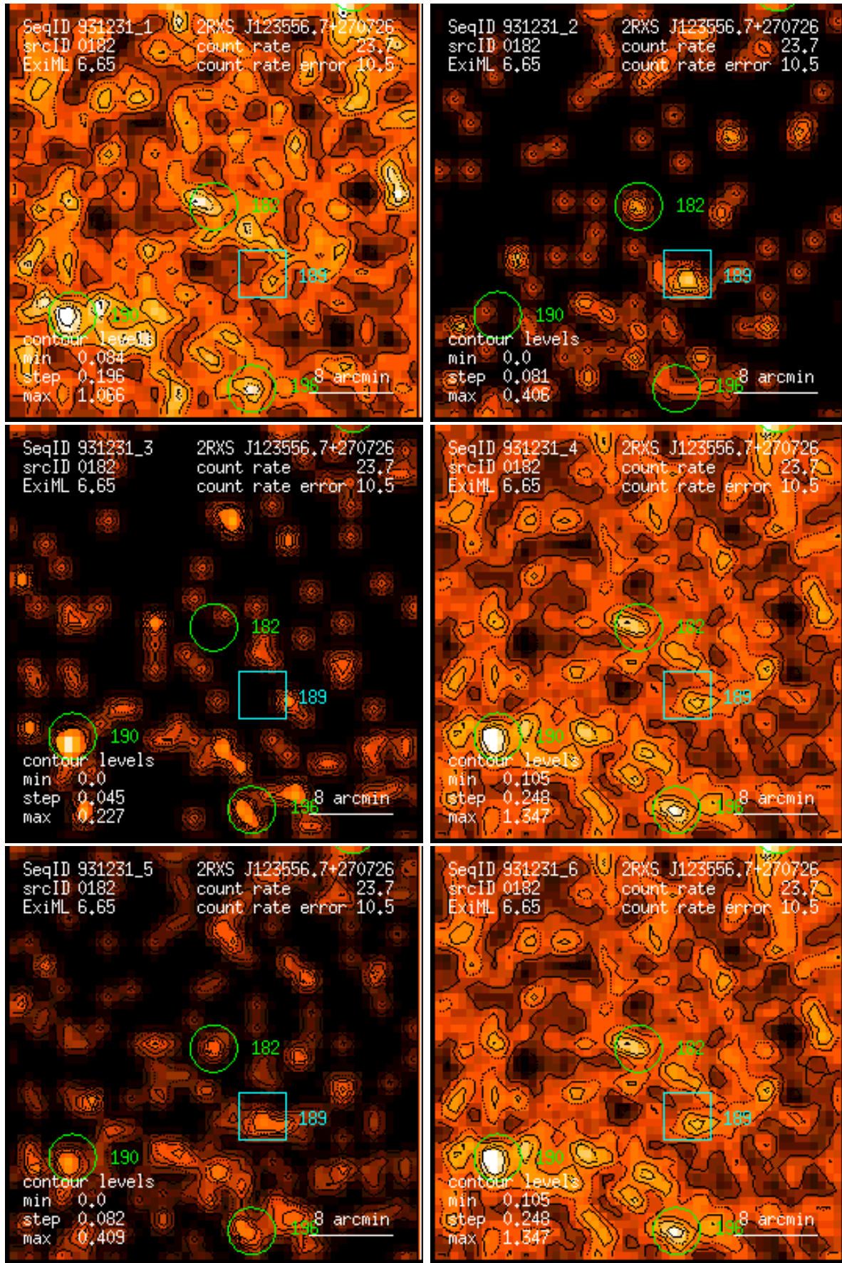
Figure 182: RASS 931231: detection 0182: band rate images, Gaussian filter: (1) PSPC channels 11 – 41, (2) 52 – 90, (3) 91 – 201, (4) 11 – 235, (5) 52 – 201, (6) 11 – 201. Broad band rates in counts/ks. Band rate contour levels in counts/ks/arcmin 2 .
