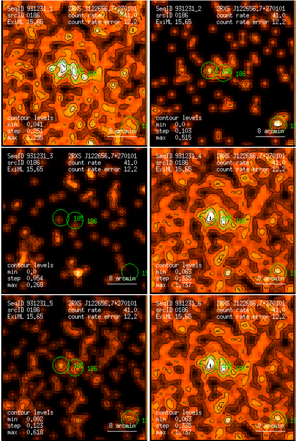
Figure 186: RASS 931231: detection 0186: band rate images, Gaussian filter: (1) PSPC channels 11 – 41, (2) 52 – 90, (3) 91 – 201, (4) 11 – 235, (5) 52 – 201, (6) 11 – 201. Broad band rates in counts/ks. Band rate contour levels in counts/ks/arcmin 2 .
