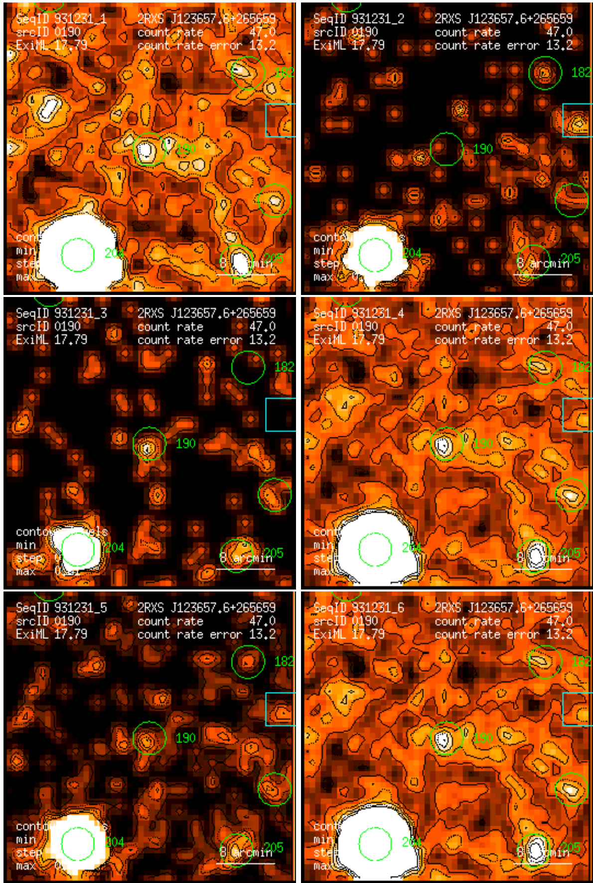
Figure 190: RASS 931231: detection 0190: band rate images, Gaussian filter: (1) PSPC channels 11 – 41, (2) 52 – 90, (3) 91 – 201, (4) 11 – 235, (5) 52 – 201, (6) 11 – 201. Broad band rates in counts/ks. Band rate contour levels in counts/ks/arcmin 2 .
