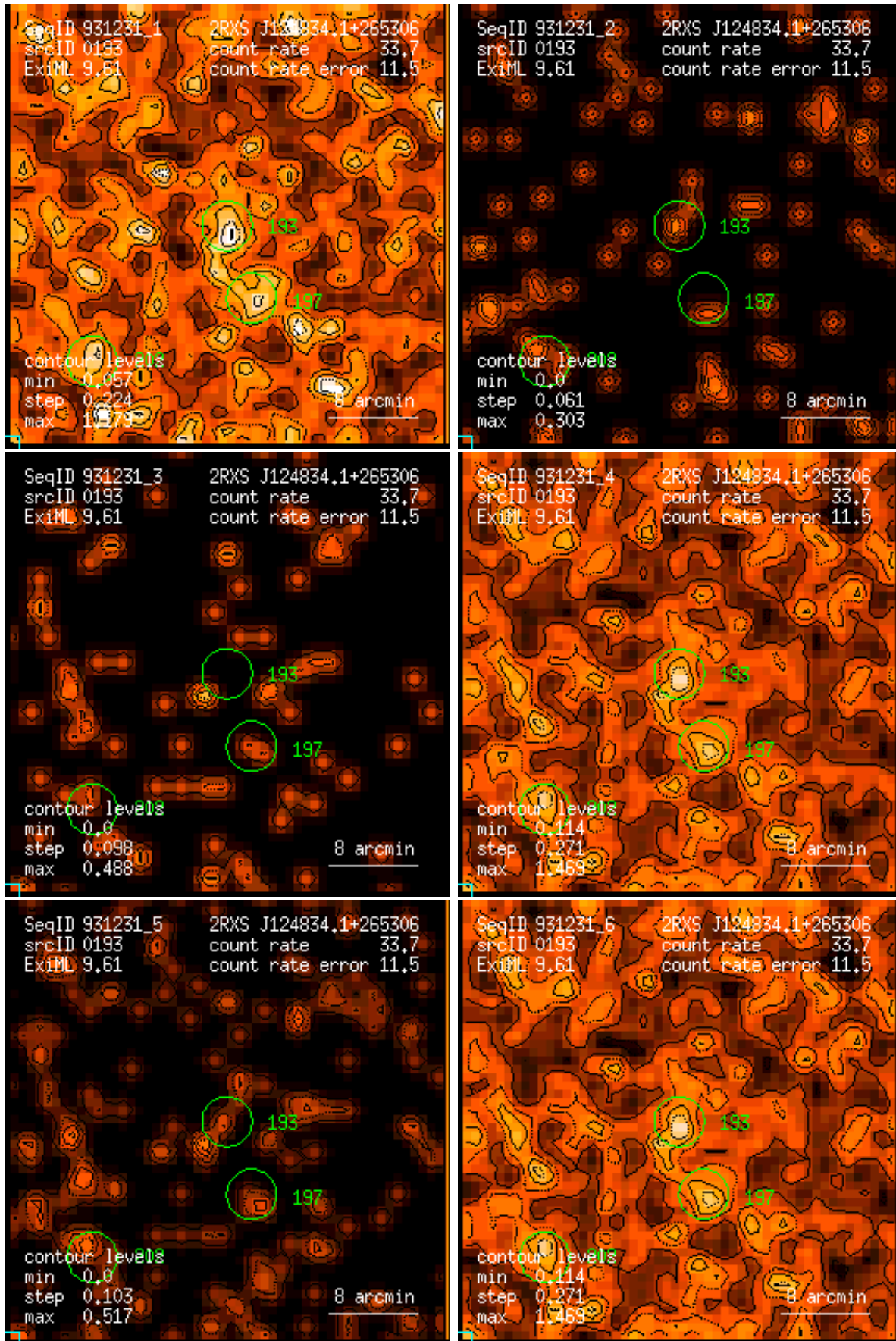
Figure 193: RASS 931231: detection 0193: band rate images, Gaussian filter: (1) PSPC channels 11 – 41, (2) 52 – 90, (3) 91 – 201, (4) 11 – 235, (5) 52 – 201, (6) 11 – 201. Broad band rates in counts/ks. Band rate contour levels in counts/ks/arcmin 2 .
