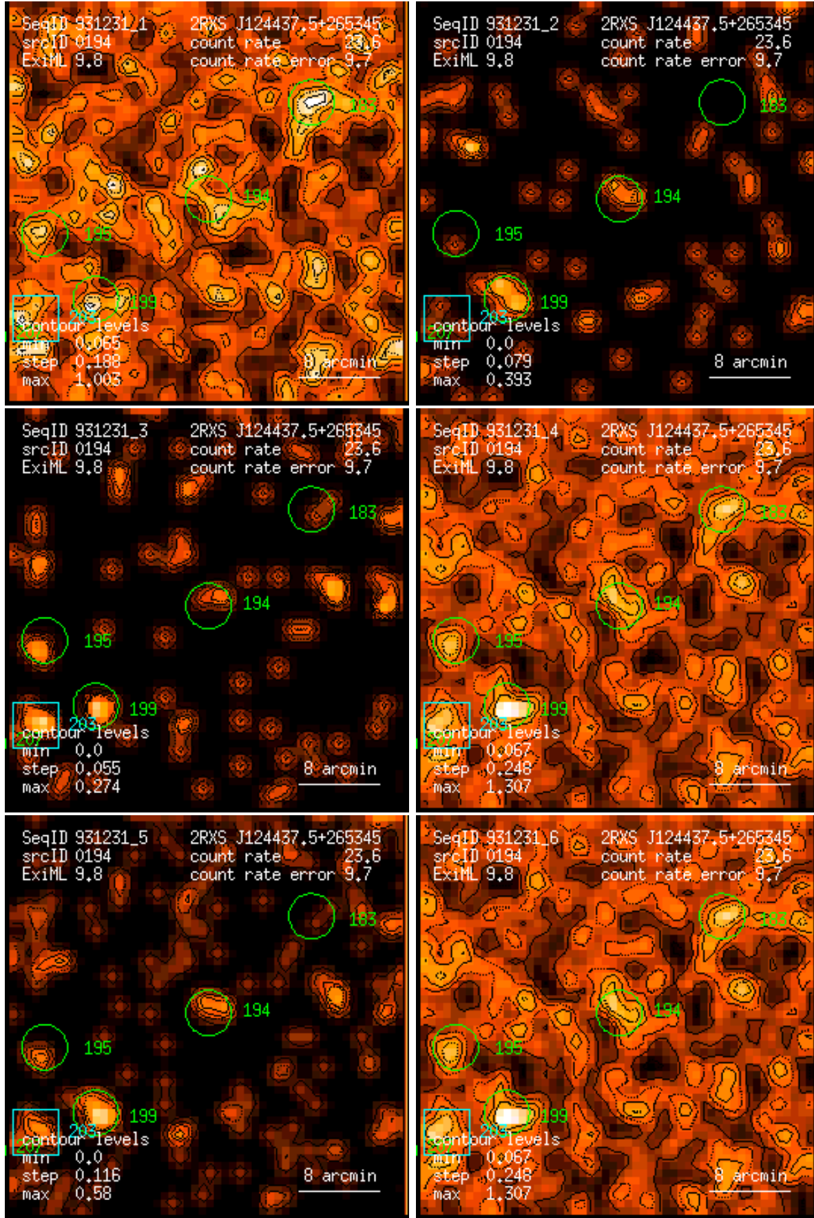
Figure 194: RASS 931231: detection 0194: band rate images, Gaussian filter: (1) PSPPC channels 11 – 41, (2) 52 – 90, (3) 91 – 201, (4) 11 – 235, (5) 52 – 201, (6) 11 – 201. Broad band rates in counts/ks. Band rate contour levels in counts/ks/arcmin 2 .
