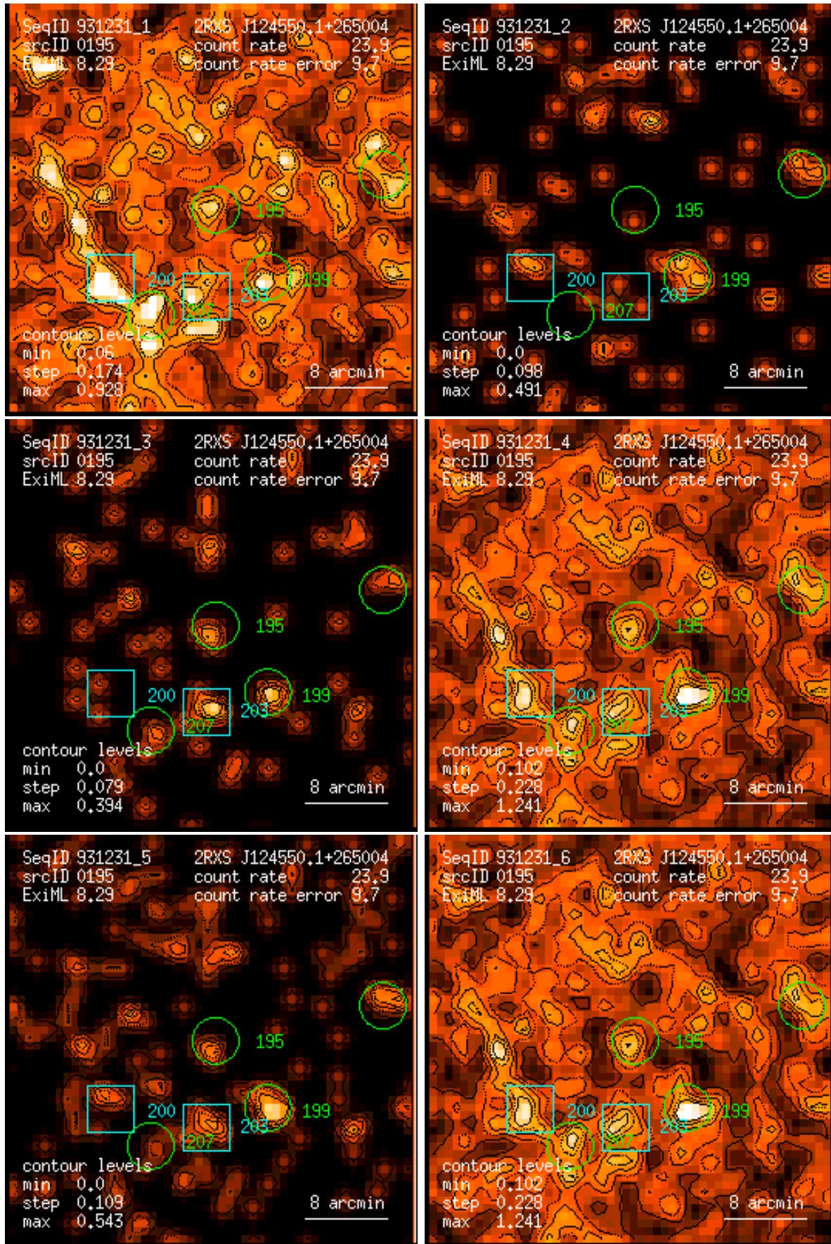
Figure 195: RASS 931231: detection 0195: band rate images, Gaussian filter: (1) PSPC channels 11 – 41, (2) 52 – 90, (3) 91 – 201, (4) 11 – 235, (5) 52 – 201, (6) 11 – 201. Broad band rates in counts/ks. Band rate contour levels in counts/ks/arcmin 2 .
