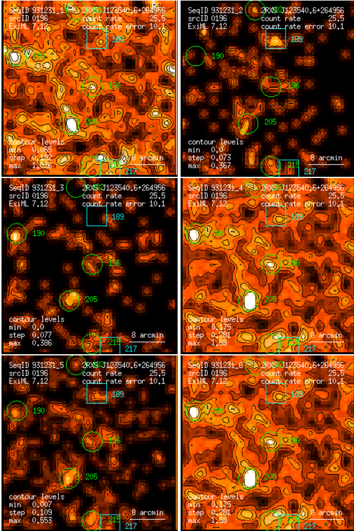
Figure 196: RASS 931231: detection 0196: band rate images, Gaussian filter: (1) PSPC channels 11 – 41, (2) 52 – 90, (3) 91 – 201, (4) 11 – 235, (5) 52 – 201, (6) 11 – 201. Broad band rates in counts/ks. Band rate contour levels in counts/ks/arcmin 2 .
