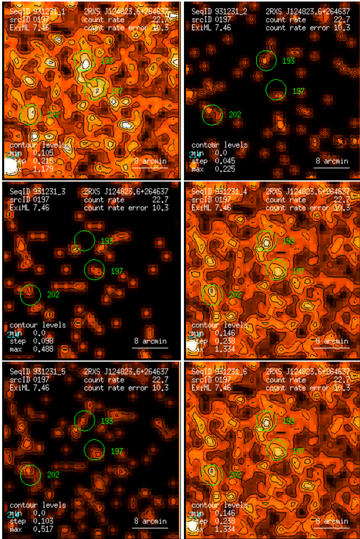
Figure 197: RASS 931231: detection 0197: band rate images, Gaussian filter: (1) PSPC channels 11 – 41, (2) 52 – 90, (3) 91 – 201, (4) 11 – 235, (5) 52 – 201, (6) 11 – 201. Broad band rates in counts/ks. Band rate contour levels in counts/ks/arcmin 2 .
