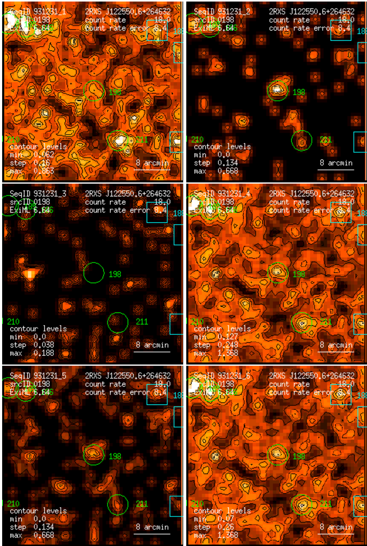
Figure 198: RASS 931231: detection 0198: band rate images, Gaussian filter: (1) PSPC channels 11 – 41, (2) 52 – 90, (3) 91 – 201, (4) 11 – 235, (5) 52 – 201, (6) 11 – 201. Broad band rates in counts/ks. Band rate contour levels in counts/ks/arcmin 2 .
