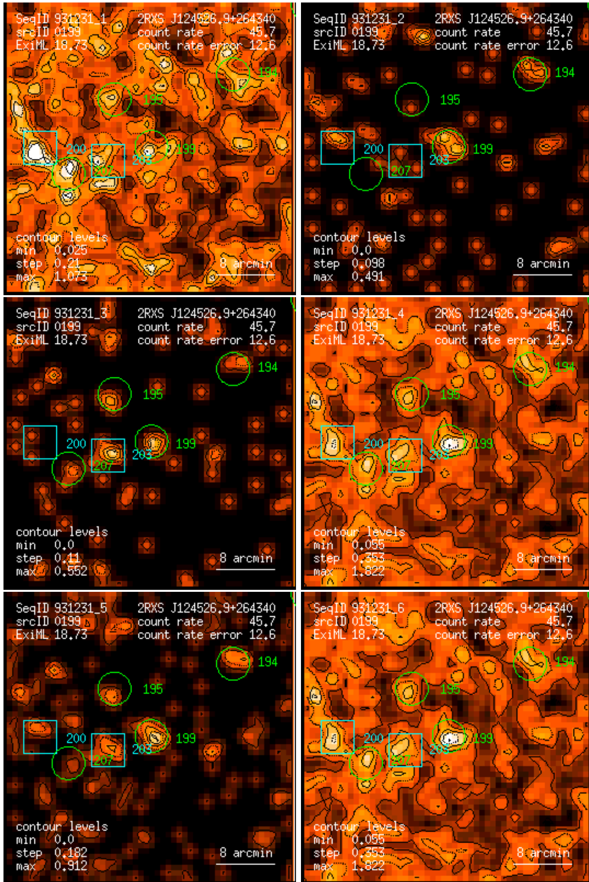
Figure 199: RASS 931231: detection 0199: band rate images, Gaussian filter: (1) PSPC channels 11 – 41, (2) 52 – 90, (3) 91 – 201, (4) 11 – 235, (5) 52 – 201, (6) 11 – 201. Broad band rates in counts/ks. Band rate contour levels in counts/ks/arcmin 2 .
