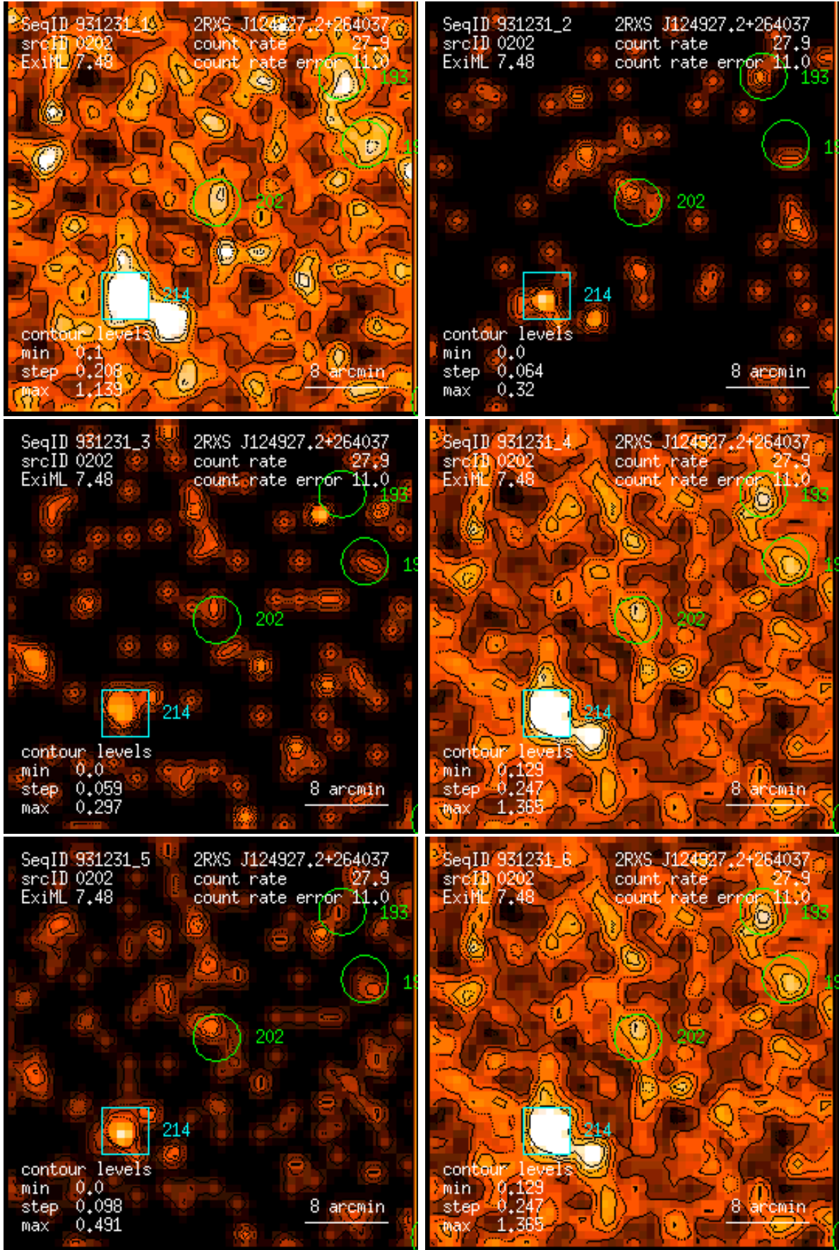
Figure 202: RASS 931231: detection 0202: band rate images, Gaussian filter: (1) PSPC channels 11 – 41, (2) 52 – 90, (3) 91 – 201, (4) 11 – 235, (5) 52 – 201, (6) 11 – 201. Broad band rates in counts/ks. Band rate contour levels in counts/ks/arcmin 2 .
