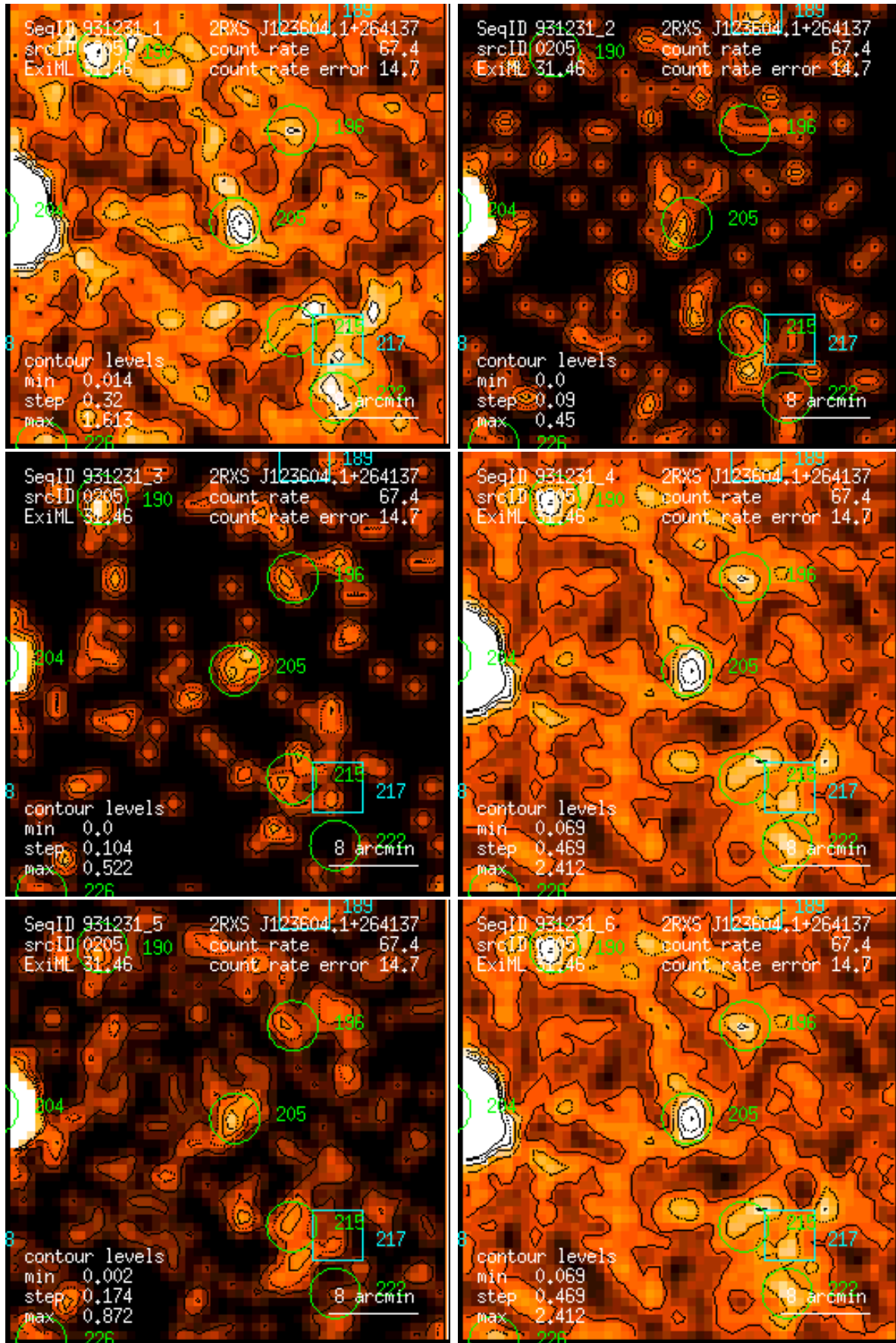
Figure 205: RASS 931231: detection 0205: band rate images, Gaussian filter: (1) PSPC channels 11 – 41, (2) 52 – 90, (3) 91 – 201, (4) 11 – 235, (5) 52 – 201, (6) 11 – 201. Broad band rates in counts/ks. Band rate contour levels in counts/ks/arcmin 2 .
