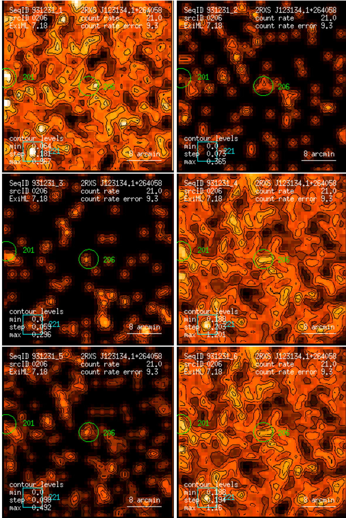
Figure 206: RASS 931231: detection 0206: band rate images, Gaussian filter: (1) PSPC channels 11 – 41, (2) 52 – 90, (3) 91 – 201, (4) 11 – 235, (5) 52 – 201, (6) 11 – 201. Broad band rates in counts/ks. Band rate contour levels in counts/ks/arcmin 2 .
