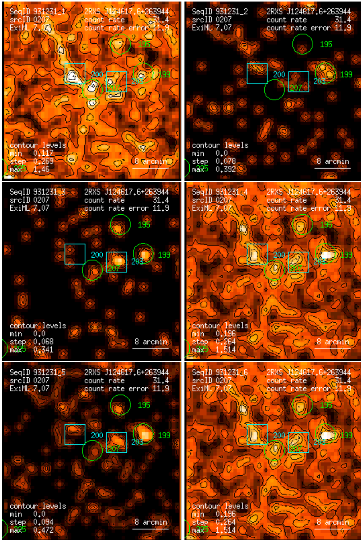
Figure 207: RASS 931231: detection 0207: band rate images, Gaussian filter: (1) PSPC channels 11 – 41, (2) 52 – 90, (3) 91 – 201, (4) 11 – 235, (5) 52 – 201, (6) 11 – 201. Broad band rates in counts/ks. Band rate contour levels in counts/ks/arcmin 2 .
