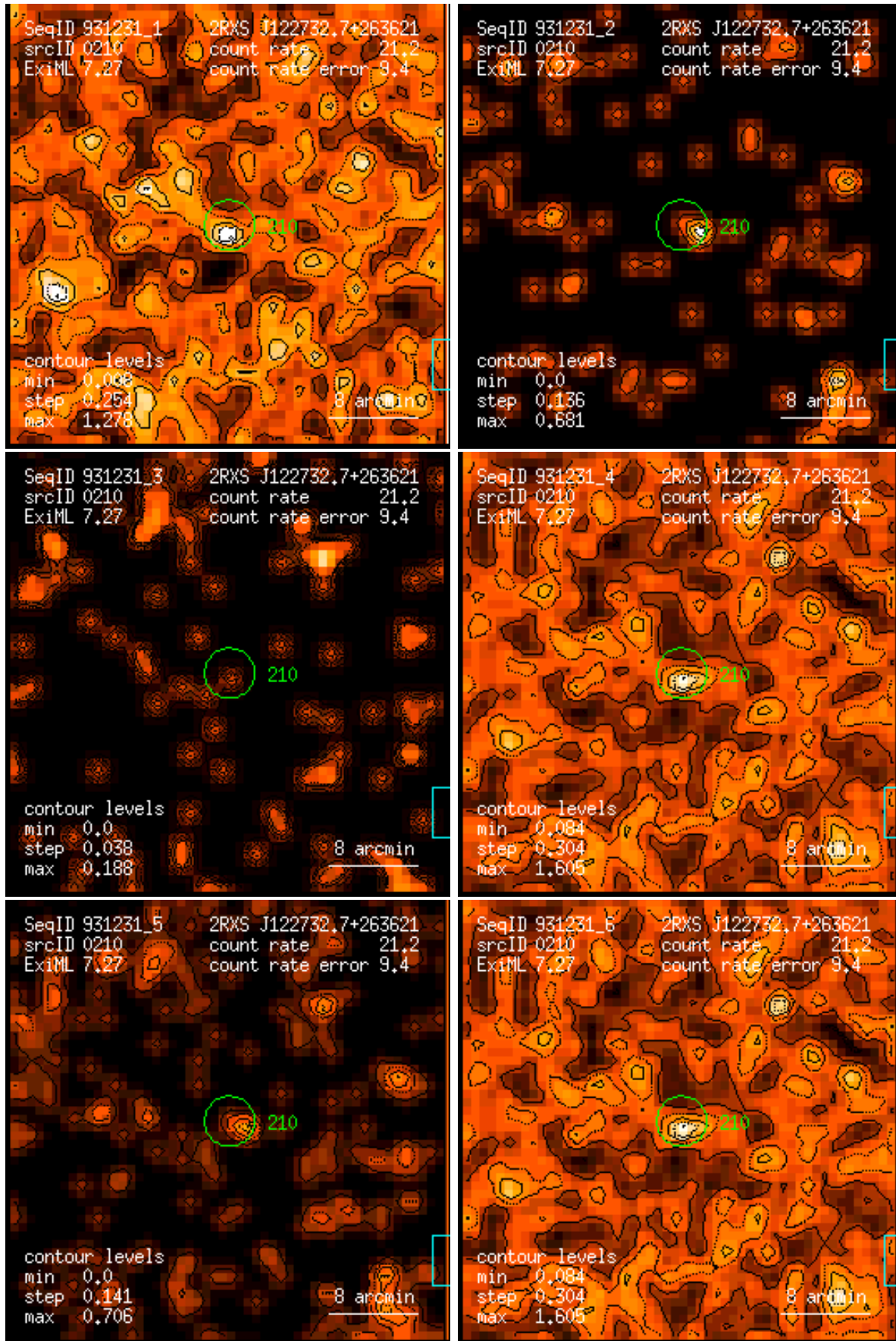
Figure 210: RASS 931231: detection 0210: band rate images, Gaussian filter: (1) PSPC channels 11 – 41, (2) 52 – 90, (3) 91 – 201, (4) 11 – 235, (5) 52 – 201, (6) 11 – 201. Broad band rates in counts/ks. Band rate contour levels in counts/ks/arcmin 2 .
