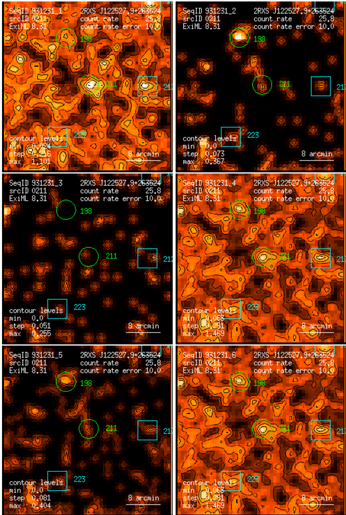
Figure 211: RASS 931231: detection 0211: band rate images, Gaussian filter: (1) PSPC channels 11 – 41, (2) 52 – 90, (3) 91 – 201, (4) 11 – 235, (5) 52 – 201, (6) 11 – 201. Broad band rates in counts/ks. Band rate contour levels in counts/ks/arcmin 2 .
