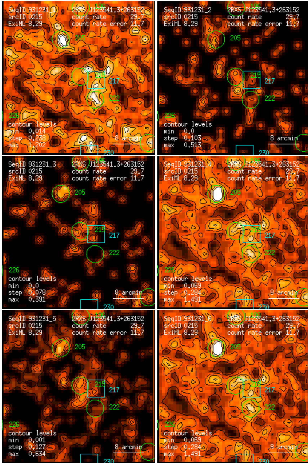
Figure 215: RASS 931231: detection 0215: band rate images, Gaussian filter: (1) PSPC channels 11 – 41, (2) 52 – 90, (3) 91 – 201, (4) 11 – 235, (5) 52 – 201, (6) 11 – 201. Broad band rates in counts/ks. Band rate contour levels in counts/ks/arcmin 2 .
