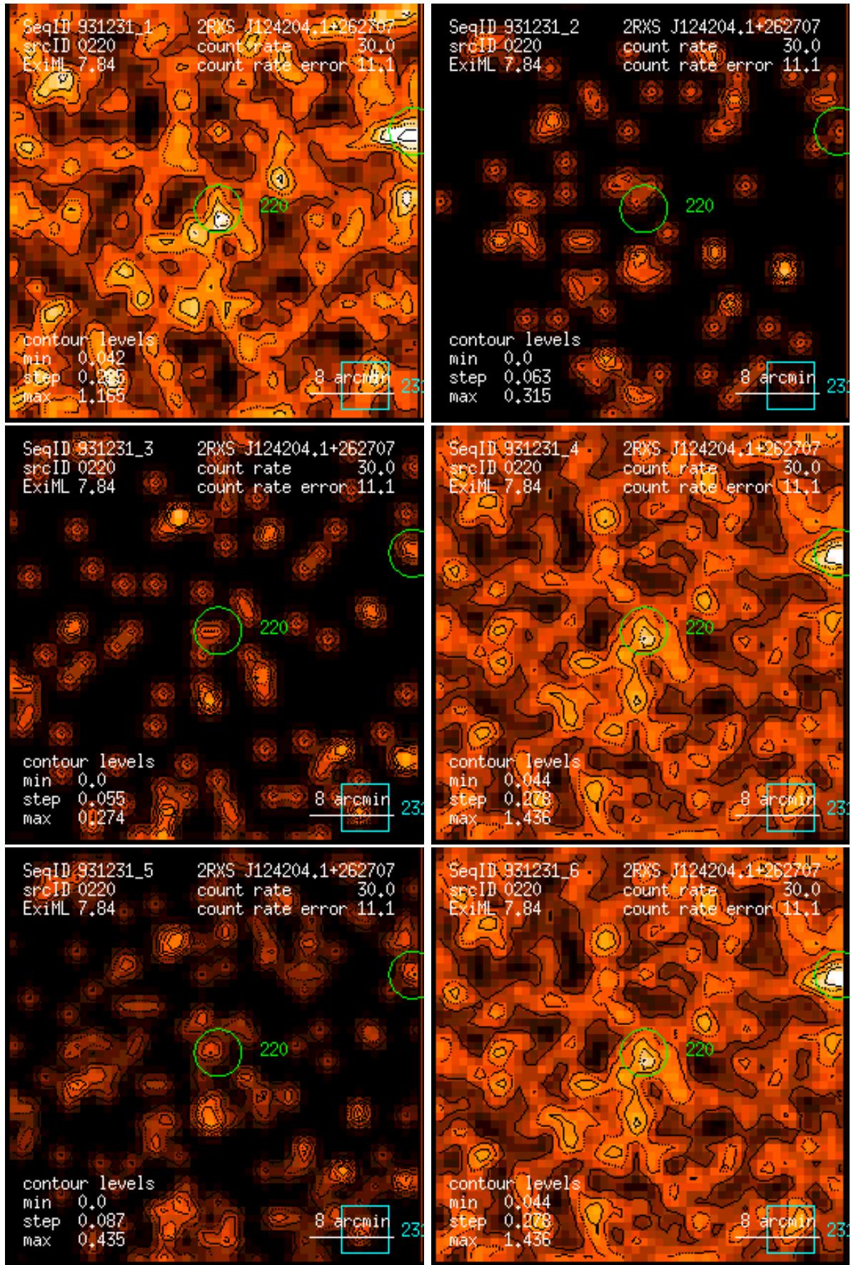
Figure 220: RASS 931231: detection 0220: band rate images, Gaussian filter: (1) PSPC channels 11 – 41, (2) 52 – 90, (3) 91 – 201, (4) 11 – 235, (5) 52 – 201, (6) 11 – 201. Broad band rates in counts/ks. Band rate contour levels in counts/ks/arcmin 2 .
