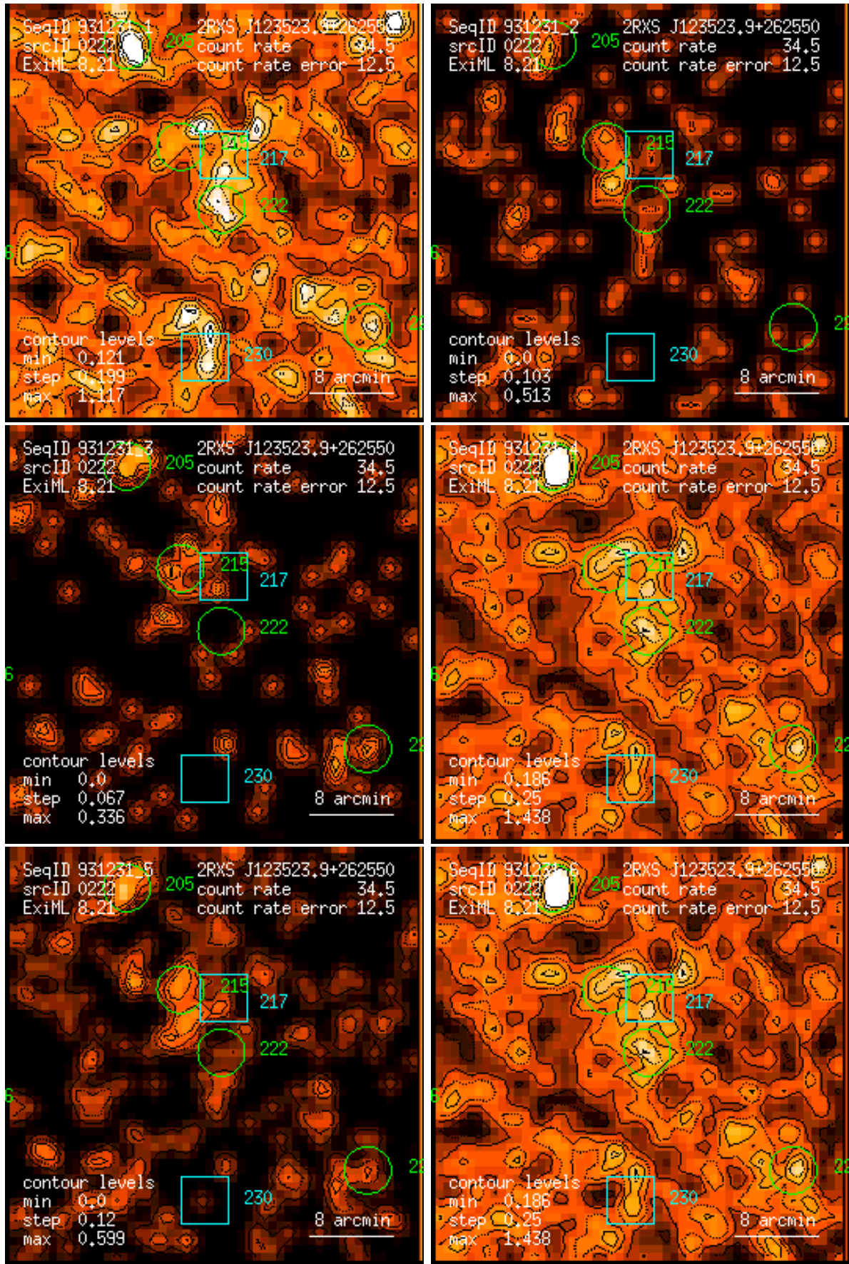
Figure 222: RASS 931231: detection 0222: band rate images, Gaussian filter: (1) PSPC channels 11 – 41, (2) 52 – 90, (3) 91 – 201, (4) 11 – 235, (5) 52 – 201, (6) 11 – 201. Broad band rates in counts/ks. Band rate contour levels in counts/ks/arcmin 2 .
