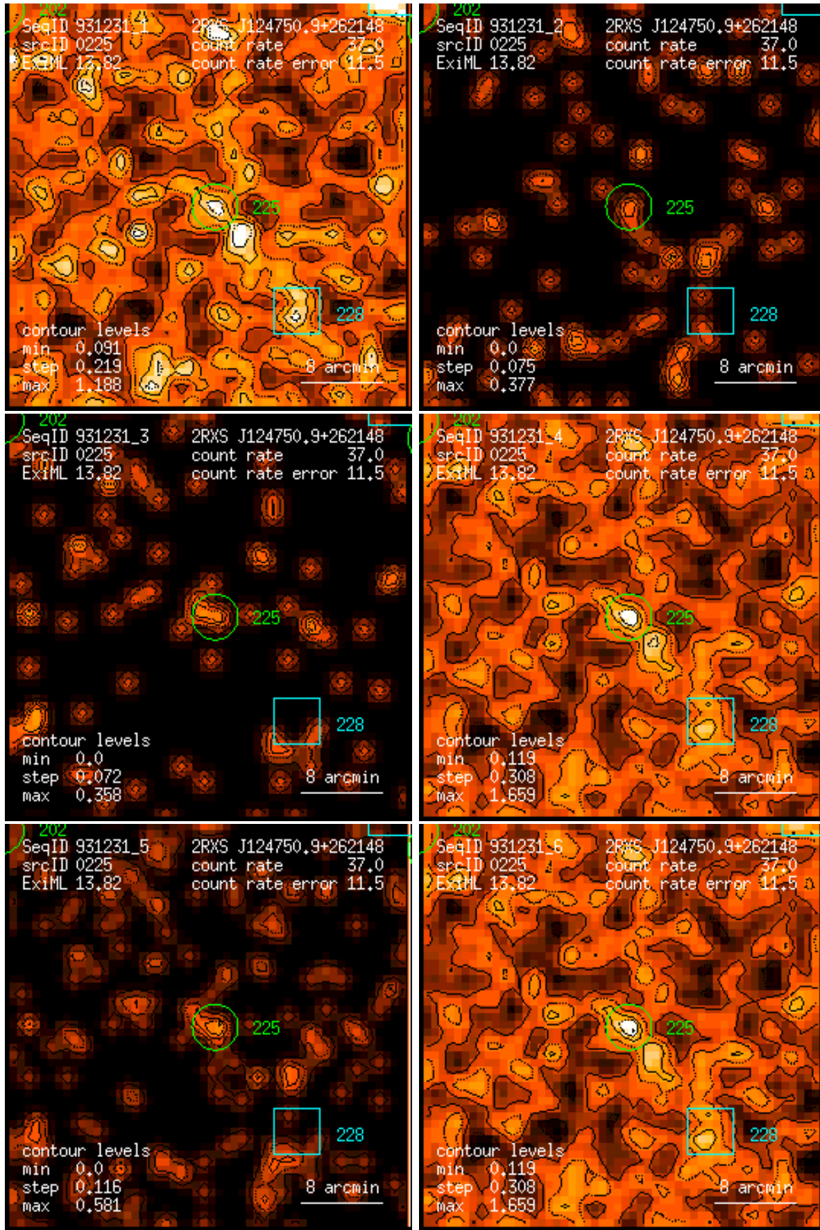
Figure 225: RASS 931231: detection 0225: band rate images, Gaussian filter: (1) PSPC channels 11 – 41, (2) 52 – 90, (3) 91 – 201, (4) 11 – 235, (5) 52 – 201, (6) 11 – 201. Broad band rates in counts/ks. Band rate contour levels in counts/ks/arcmin 2 .
