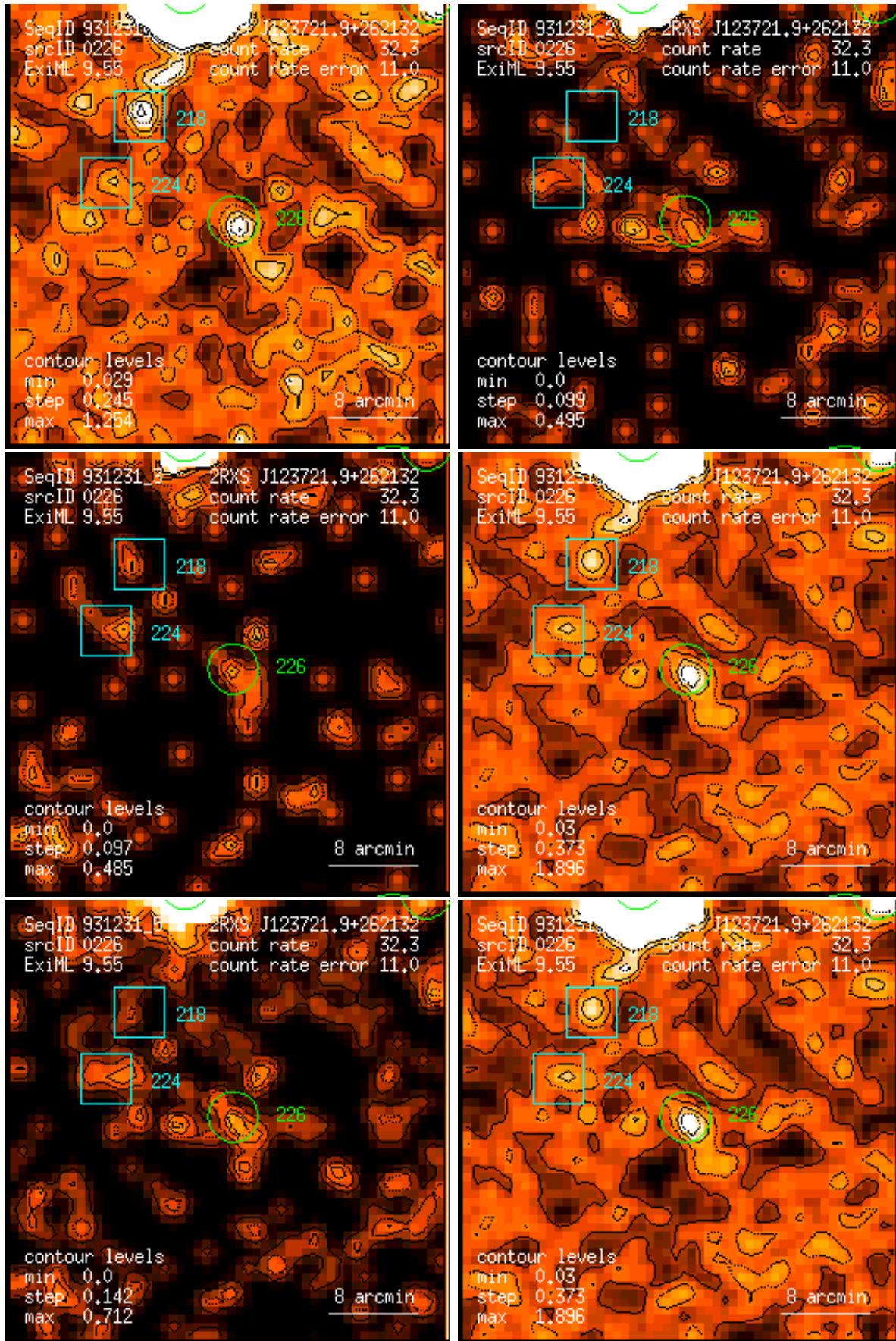
Figure 226: RASS 931231: detection 0226: band rate images, Gaussian filter: (1) PSPC channels 11 – 41, (2) 52 – 90, (3) 91 – 201, (4) 11 – 235, (5) 52 – 201, (6) 11 – 201. Broad band rates in counts/ks. Band rate contour levels in counts/ks/arcmin 2 .
