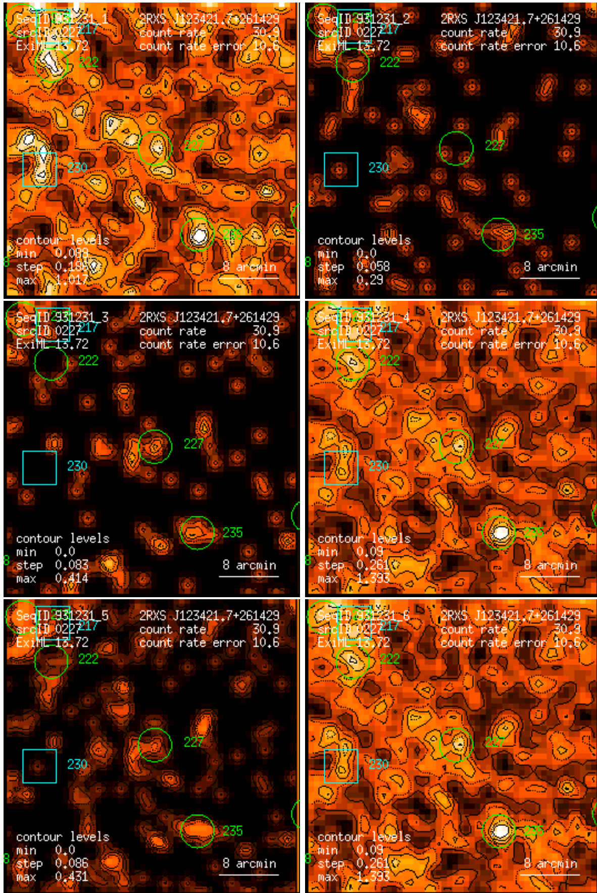
Figure 227: RASS 931231: detection 0227: band rate images, Gaussian filter: (1) PSPC channels 11 – 41, (2) 52 – 90, (3) 91 – 201, (4) 11 – 235, (5) 52 – 201, (6) 11 – 201. Broad band rates in counts/ks. Band rate contour levels in counts/ks/arcmin 2 .
