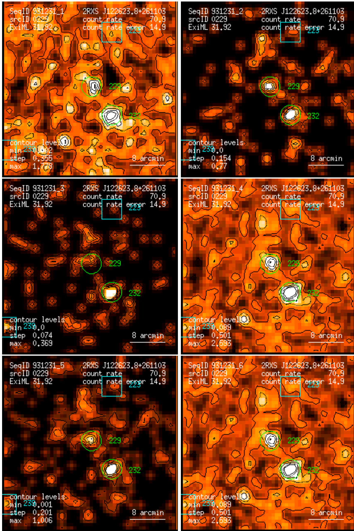
Figure 229: RASS 931231: detection 0229: band rate images, Gaussian filter: (1) PSPC channels 11 – 41, (2) 52 – 90, (3) 91 – 201, (4) 11 – 235, (5) 52 – 201, (6) 11 – 201. Broad band rates in counts/ks. Band rate contour levels in counts/ks/arcmin 2 .
