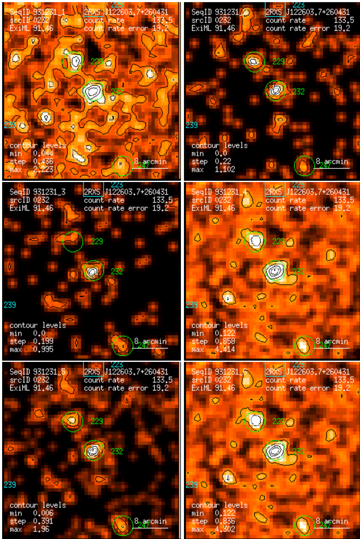
Figure 232: RASS 931231: detection 0232: band rate images, Gaussian filter: (1) PSPC channels 11 – 41, (2) 52 – 90, (3) 91 – 201, (4) 11 – 235, (5) 52 – 201, (6) 11 – 201. Broad band rates in counts/ks. Band rate contour levels in counts/ks/arcmin 2 .
