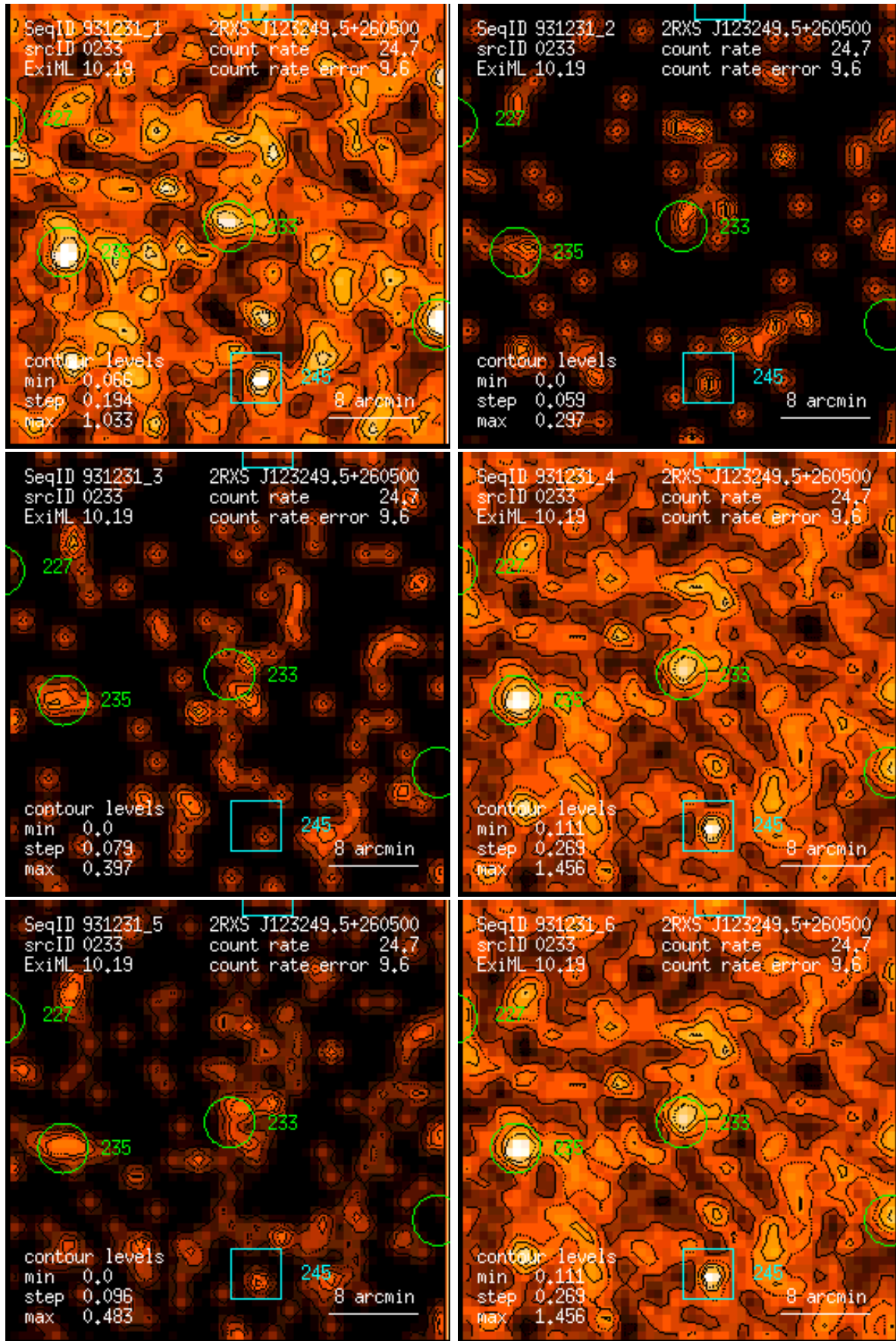
Figure 233: RASS 931231: detection 0233: band rate images, Gaussian filter: (1) PSPC channels 11 – 41, (2) 52 – 90, (3) 91 – 201, (4) 11 – 235, (5) 52 – 201, (6) 11 – 201. Broad band rates in counts/ks. Band rate contour levels in counts/ks/arcmin 2 .
