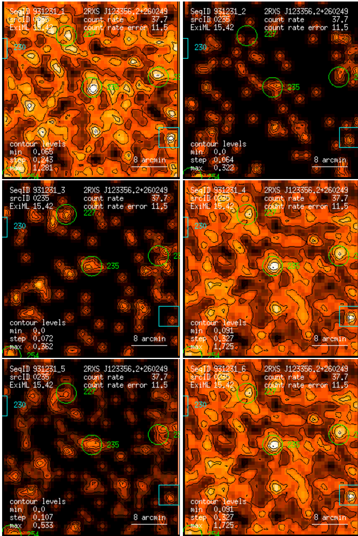
Figure 235: RASS 931231: detection 0235: band rate images, Gaussian filter: (1) PSPC channels 11 – 41, (2) 52 – 90, (3) 91 – 201, (4) 11 – 235, (5) 52 – 201, (6) 11 – 201. Broad band rates in counts/ks. Band rate contour levels in counts/ks/arcmin 2 .
