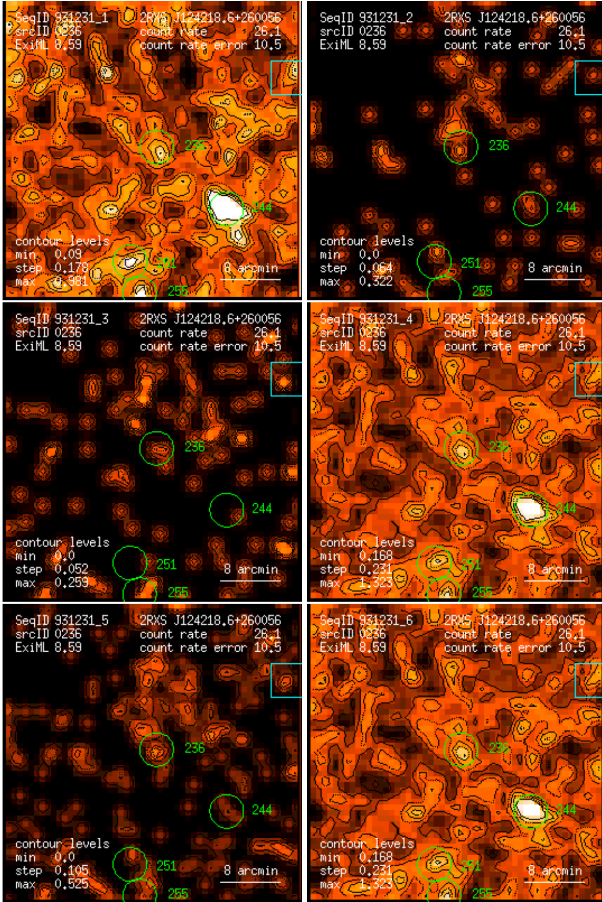
Figure 236: RASS 931231: detection 0236: band rate images, Gaussian filter: (1) PSPC channels 11 – 41, (2) 52 – 90, (3) 91 – 201, (4) 11 – 235, (5) 52 – 201, (6) 11 – 201. Broad band rates in counts/ks. Band rate contour levels in counts/ks/arcmin 2 .
