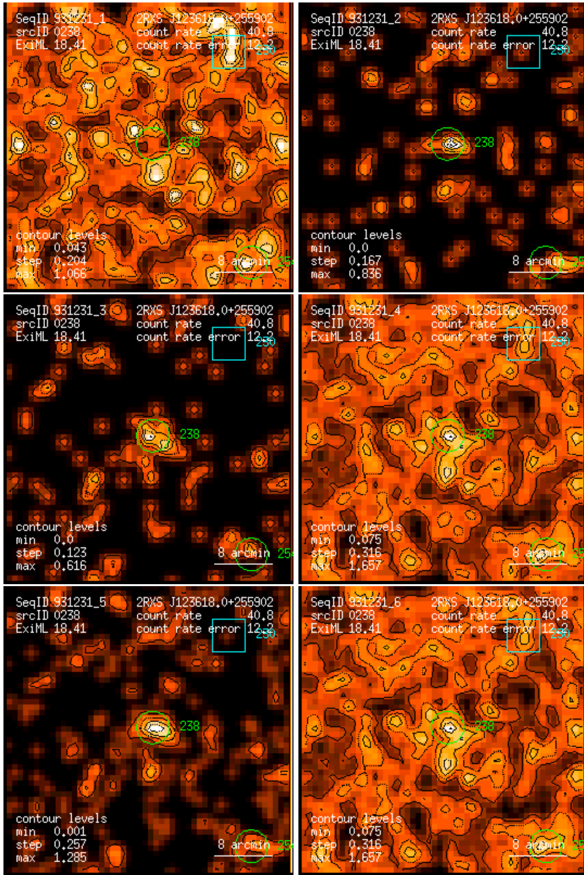
Figure 238: RASS 931231: detection 0238: band rate images, Gaussian filter: (1) PSPC channels 11 – 41, (2) 52 – 90, (3) 91 – 201, (4) 11 – 235, (5) 52 – 201, (6) 11 – 201. Broad band rates in counts/ks. Band rate contour levels in counts/ks/arcmin 2 .
