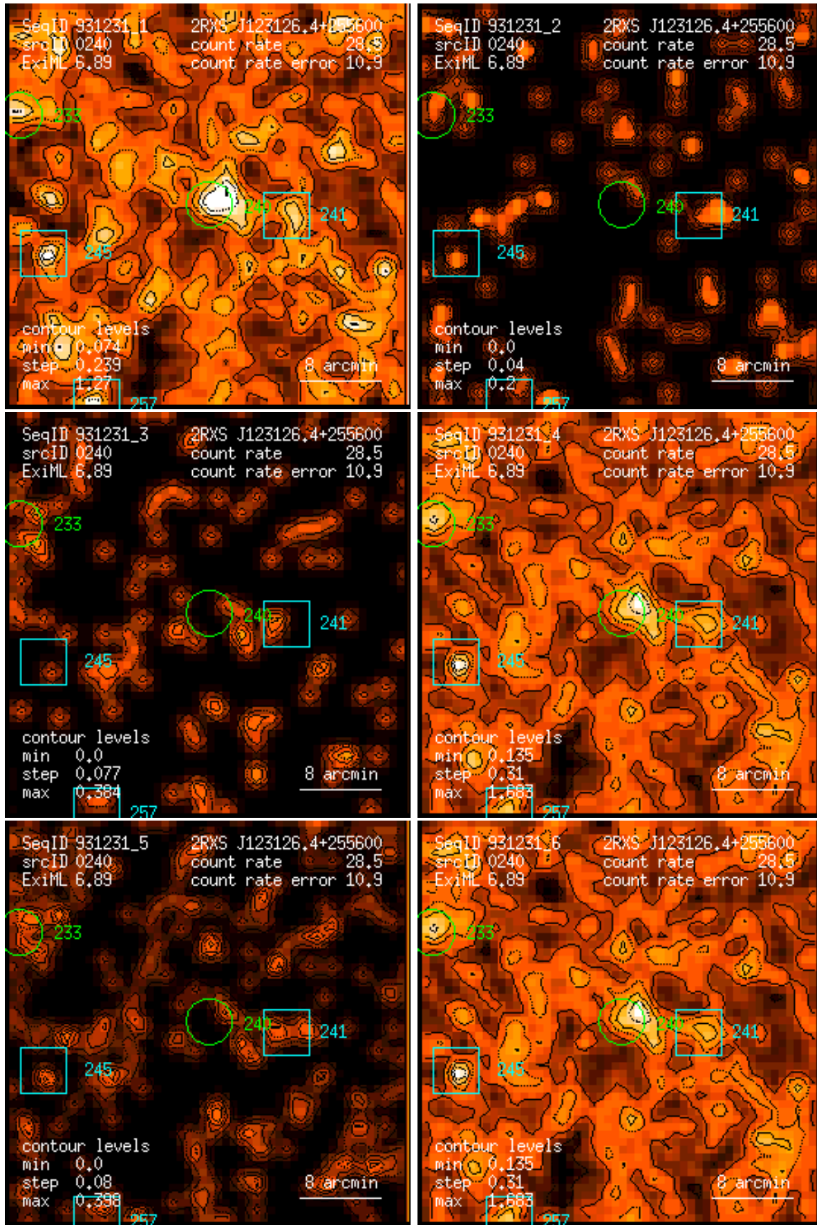
Figure 240: RASS 931231: detection 0240: band rate images, Gaussian filter: (1) PSPC channels 11 – 41, (2) 52 – 90, (3) 91 – 201, (4) 11 – 235, (5) 52 – 201, (6) 11 – 201. Broad band rates in counts/ks. Band rate contour levels in counts/ks/arcmin 2 .
