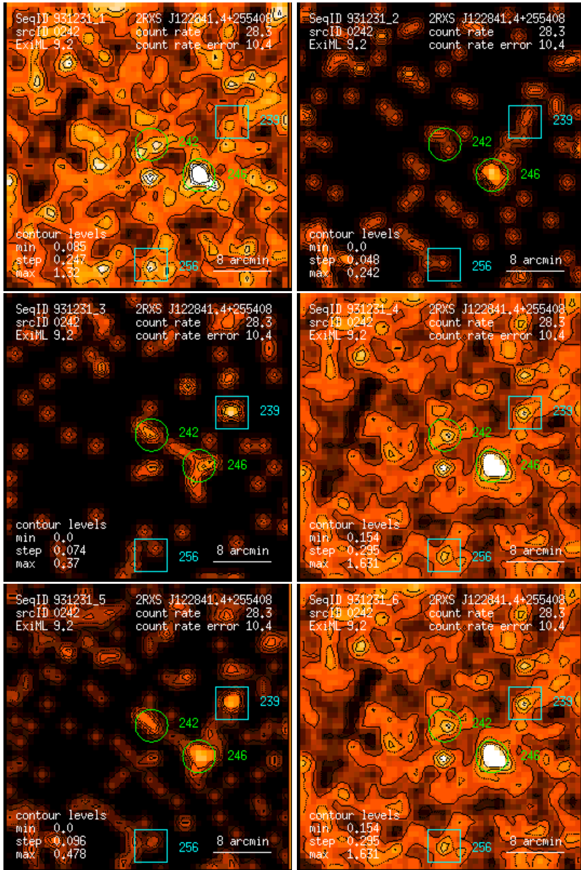
Figure 242: RASS 931231: detection 0242: band rate images, Gaussian filter: (1) PSPC channels 11 – 41, (2) 52 – 90, (3) 91 – 201, (4) 11 – 235, (5) 52 – 201, (6) 11 – 201. Broad band rates in counts/ks. Band rate contour levels in counts/ks/arcmin 2 .
