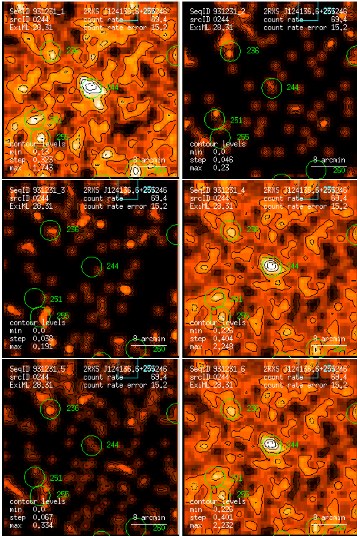
Figure 244: RASS 931231: detection 0244: band rate images, Gaussian filter: (1) PSPC channels 11 – 41, (2) 52 – 90, (3) 91 – 201, (4) 11 – 235, (5) 52 – 201, (6) 11 – 201. Broad band rates in counts/ks. Band rate contour levels in counts/ks/arcmin 2 .
