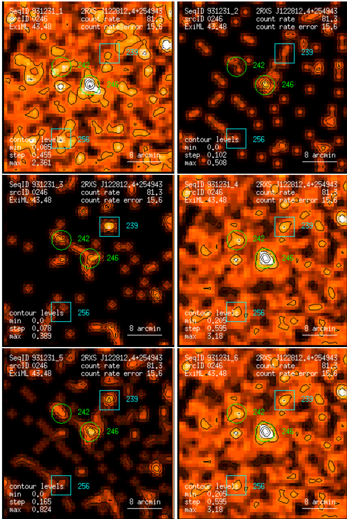
Figure 246: RASS 931231: detection 0246: band rate images, Gaussian filter: (1) PSPC channels 11 – 41, (2) 52 – 90, (3) 91 – 201, (4) 11 – 235, (5) 52 – 201, (6) 11 – 201. Broad band rates in counts/ks. Band rate contour levels in counts/ks/arcmin 2 .
