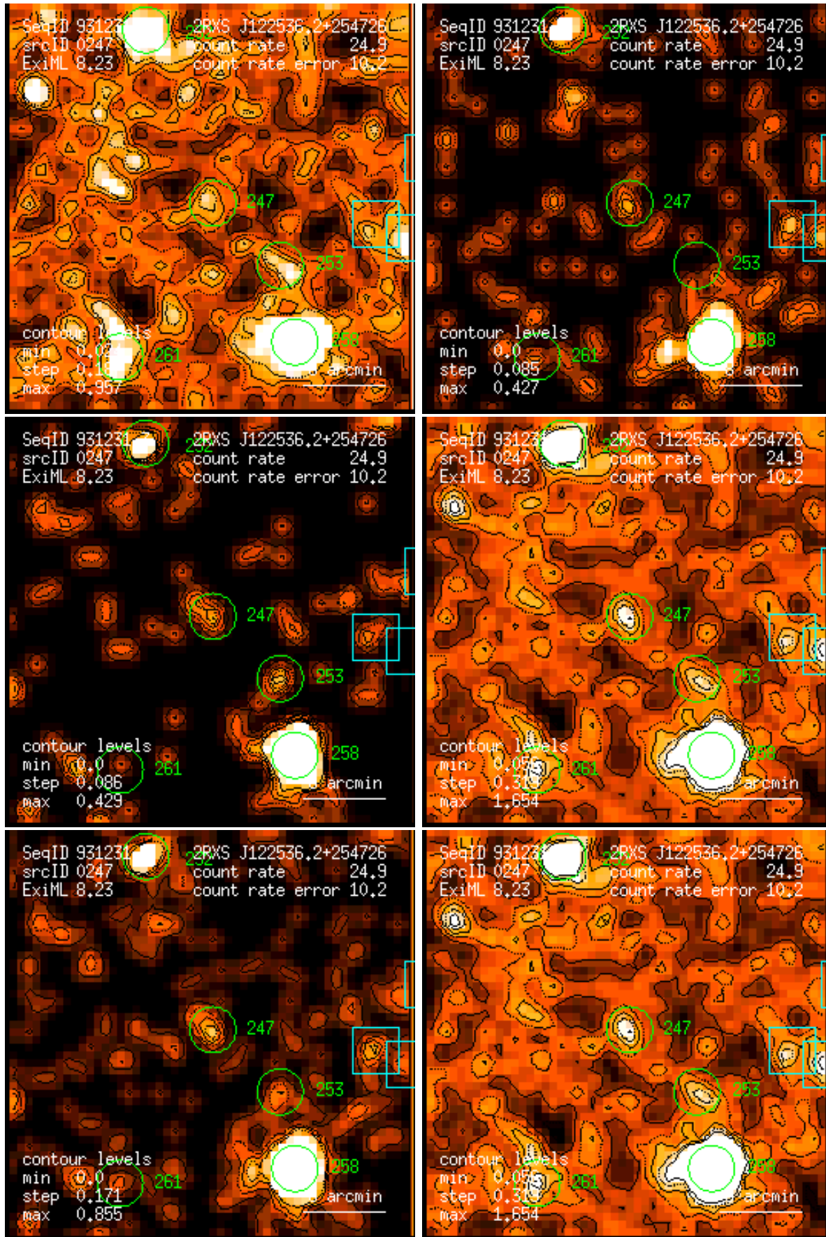
Figure 247: RASS 931231: detection 0247: band rate images, Gaussian filter: (1) PSPC channels 11 – 41, (2) 52 – 90, (3) 91 – 201, (4) 11 – 235, (5) 52 – 201, (6) 11 – 201. Broad band rates in counts/ks. Band rate contour levels in counts/ks/arcmin 2 .
