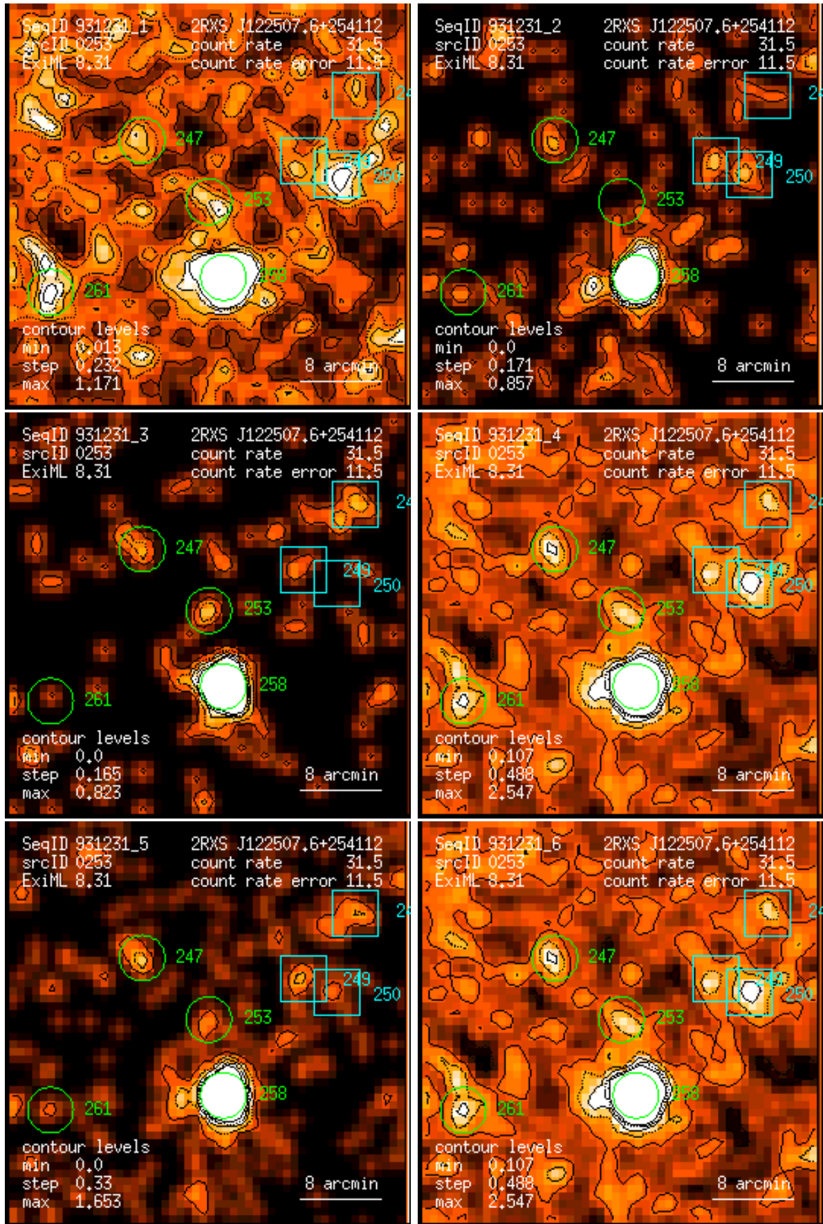
Figure 253: RASS 931231: detection 0253: band rate images, Gaussian filter: (1) PSPC channels 11 – 41, (2) 52 – 90, (3) 91 – 201, (4) 11 – 235, (5) 52 – 201, (6) 11 – 201. Broad band rates in counts/ks. Band rate contour levels in counts/ks/arcmin 2 .
