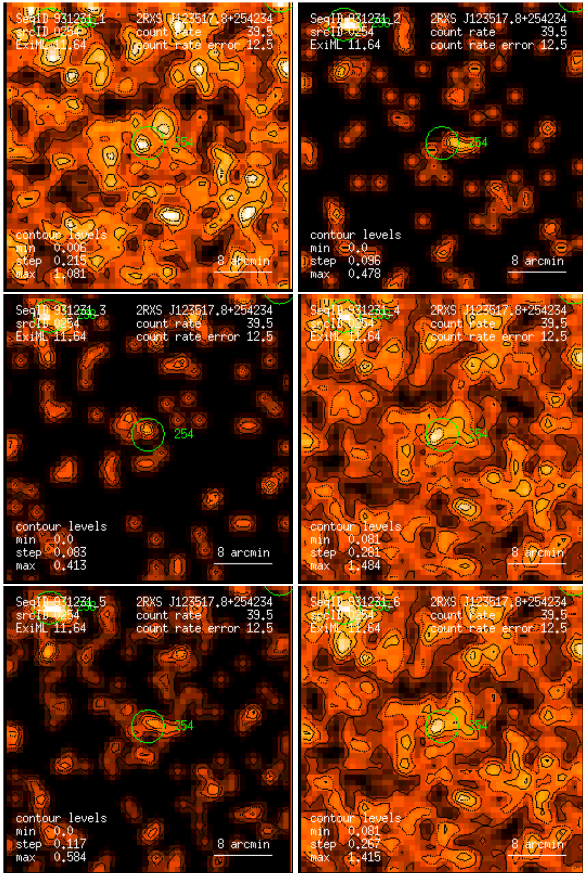
Figure 254: RASS 931231: detection 0254: band rate images, Gaussian filter: (1) PSPC channels 11 – 41, (2) 52 – 90, (3) 91 – 201, (4) 11 – 235, (5) 52 – 201, (6) 11 – 201. Broad band rates in counts/ks. Band rate contour levels in counts/ks/arcmin 2 .
