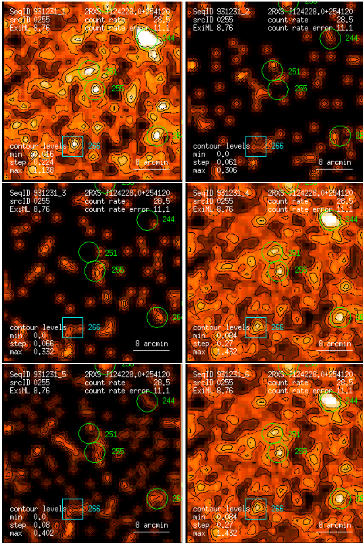
Figure 255: RASS 931231: detection 0255: band rate images, Gaussian filter: (1) PSPC channels 11 – 41, (2) 52 – 90, (3) 91 – 201, (4) 11 – 235, (5) 52 – 201, (6) 11 – 201. Broad band rates in counts/ks. Band rate contour levels in counts/ks/arcmin 2 .
