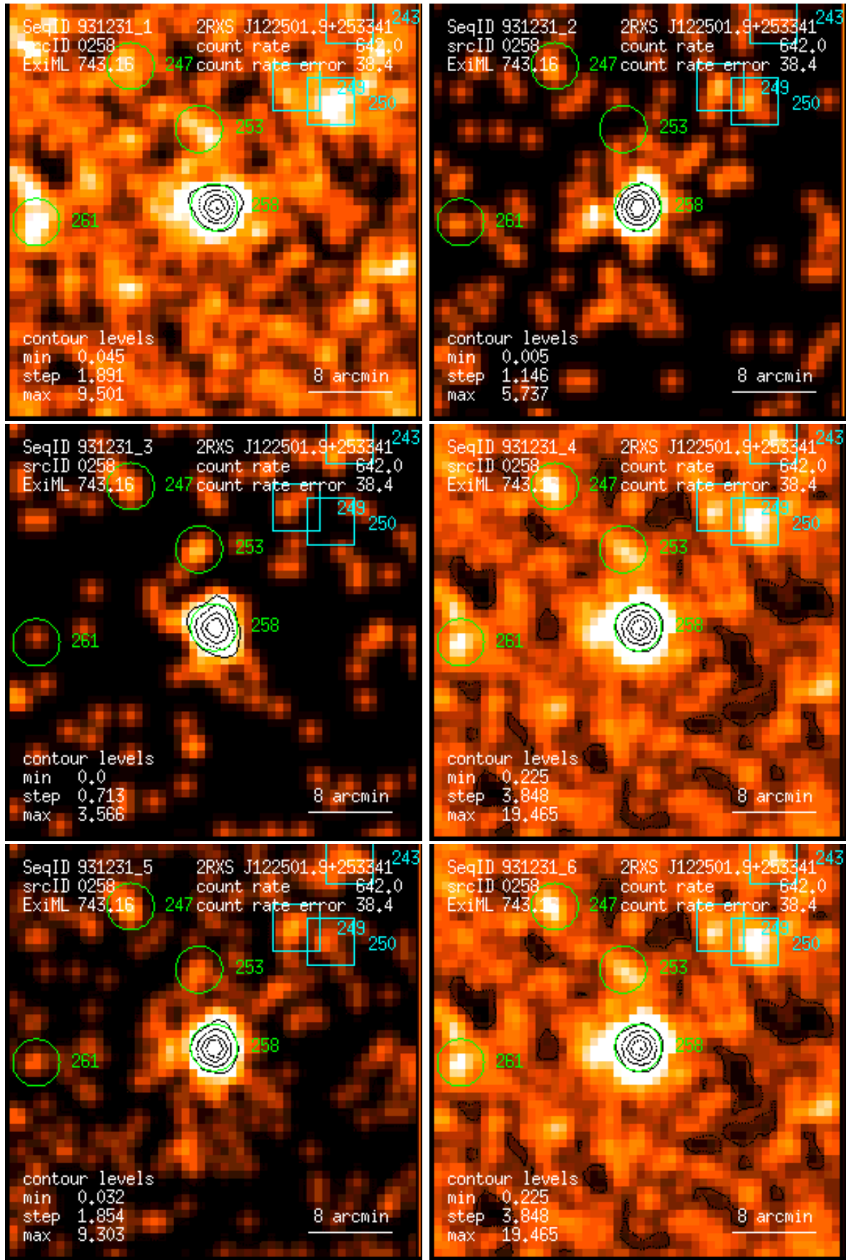
Figure 258: RASS 931231: detection 0258: band rate images, Gaussian filter: (1) PSPC channels 11 – 41, (2) 52 – 90, (3) 91 – 201, (4) 11 – 235, (5) 52 – 201, (6) 11 – 201. Broad band rates in counts/ks. Band rate contour levels in counts/ks/arcmin 2 .
