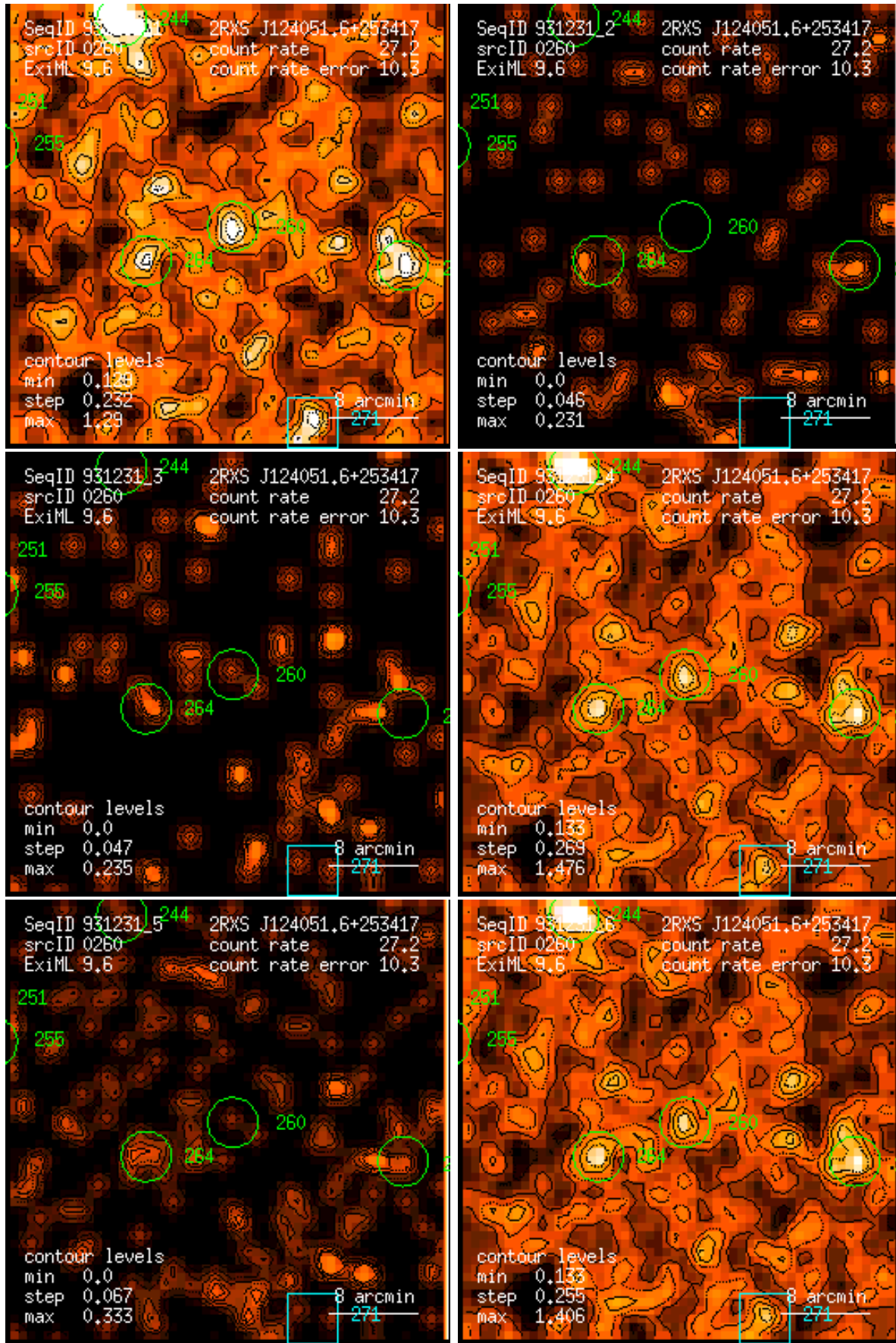
Figure 260: RASS 931231: detection 0260: band rate images, Gaussian filter: (1) PSPC channels 11 – 41, (2) 52 – 90, (3) 91 – 201, (4) 11 – 235, (5) 52 – 201, (6) 11 – 201. Broad band rates in counts/ks. Band rate contour levels in counts/ks/arcmin 2 .
