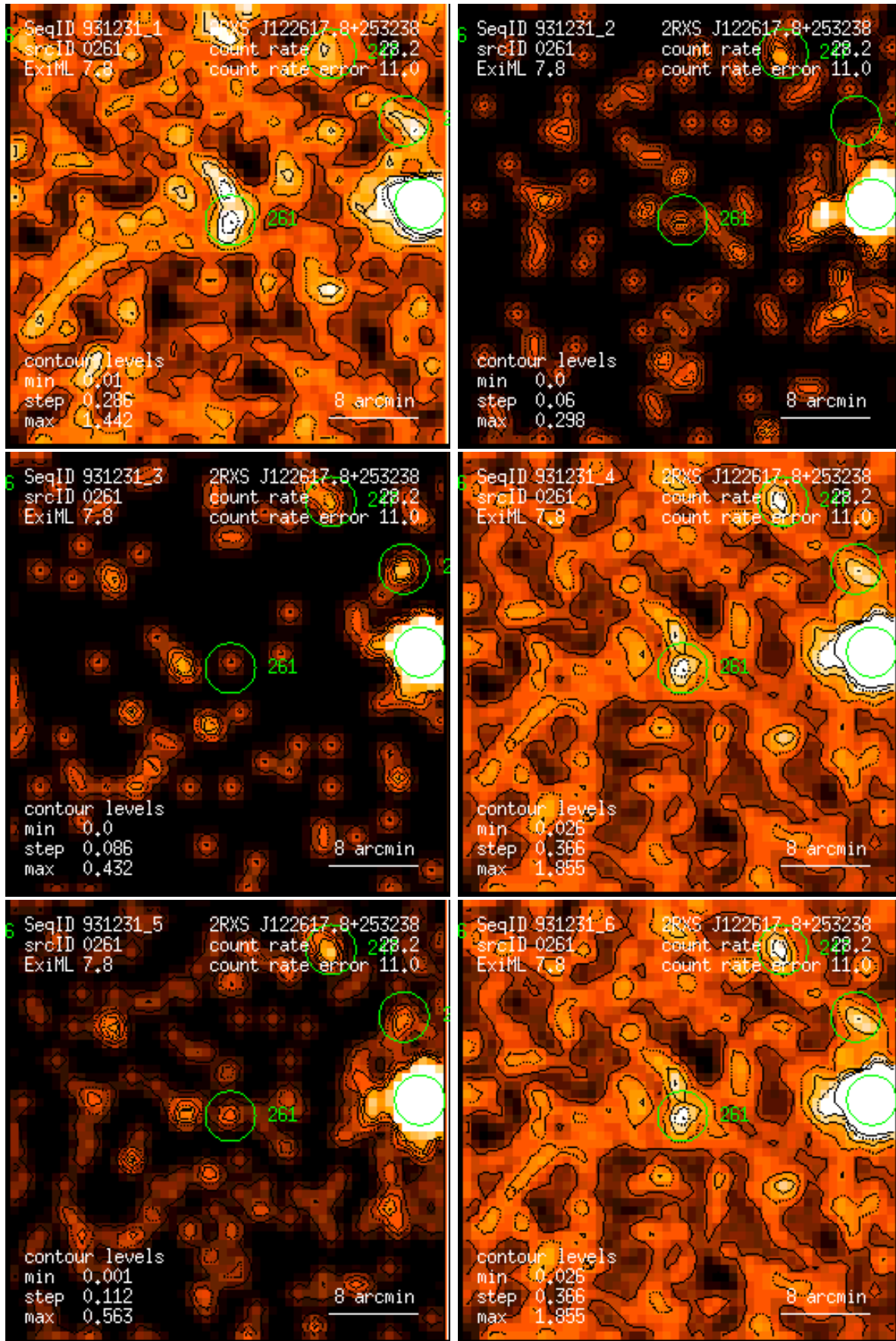
Figure 261: RASS 931231: detection 0261: band rate images, Gaussian filter: (1) PSPC channels 11 – 41, (2) 52 – 90, (3) 91 – 201, (4) 11 – 235, (5) 52 – 201, (6) 11 – 201. Broad band rates in counts/ks. Band rate contour levels in counts/ks/arcmin 2 .
