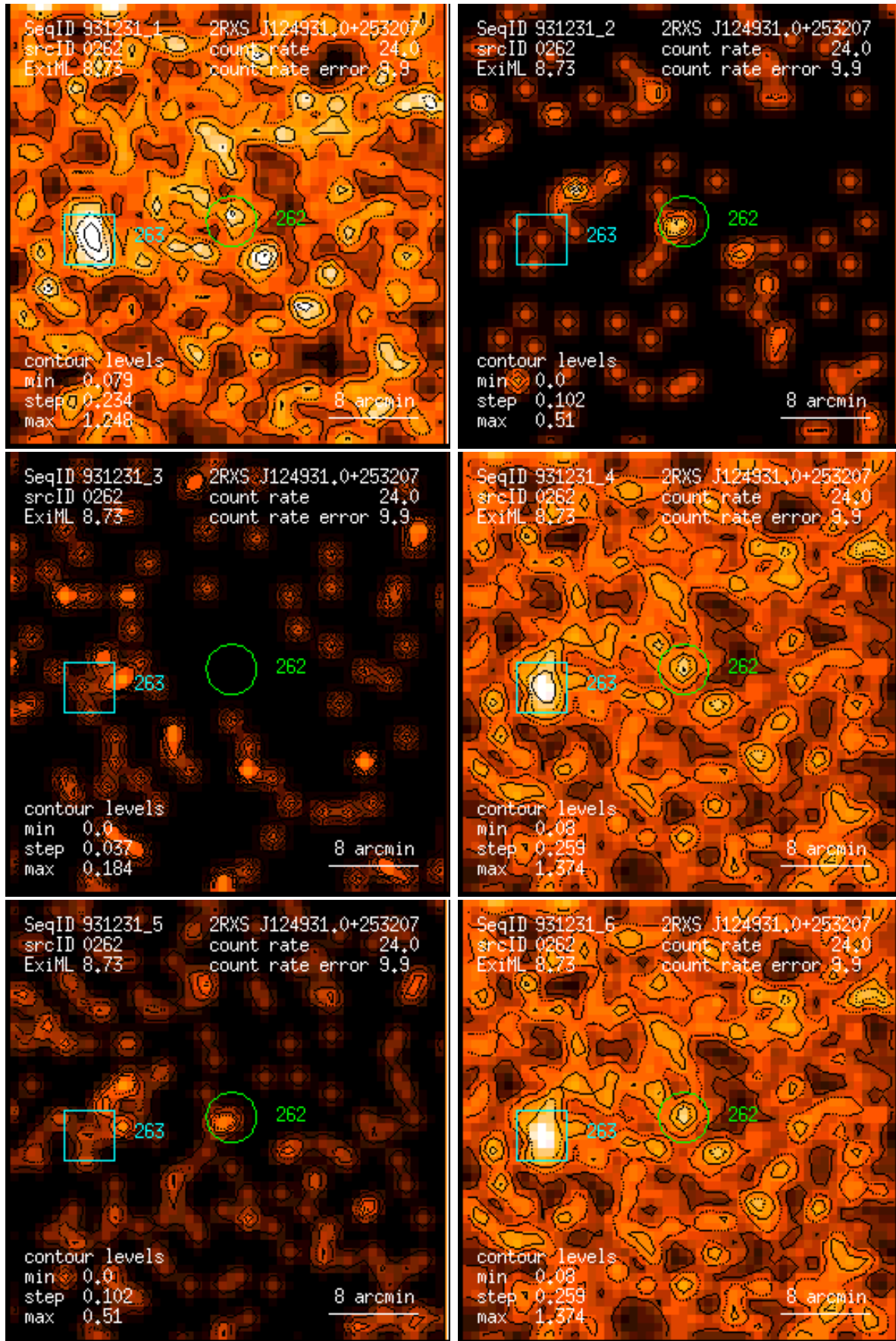
Figure 262: RASS 931231: detection 0262: band rate images, Gaussian filter: (1) PSPC channels 11 – 41, (2) 52 – 90, (3) 91 – 201, (4) 11 – 235, (5) 52 – 201, (6) 11 – 201. Broad band rates in counts/ks. Band rate contour levels in counts/ks/arcmin 2 .
