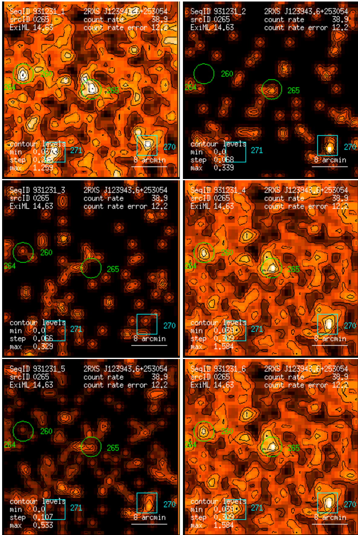
Figure 265: RASS 931231: detection 0265: band rate images, Gaussian filter: (1) PSPC channels 11 – 41, (2) 52 – 90, (3) 91 – 201, (4) 11 – 235, (5) 52 – 201, (6) 11 – 201. Broad band rates in counts/ks. Band rate contour levels in counts/ks/arcmin 2 .
