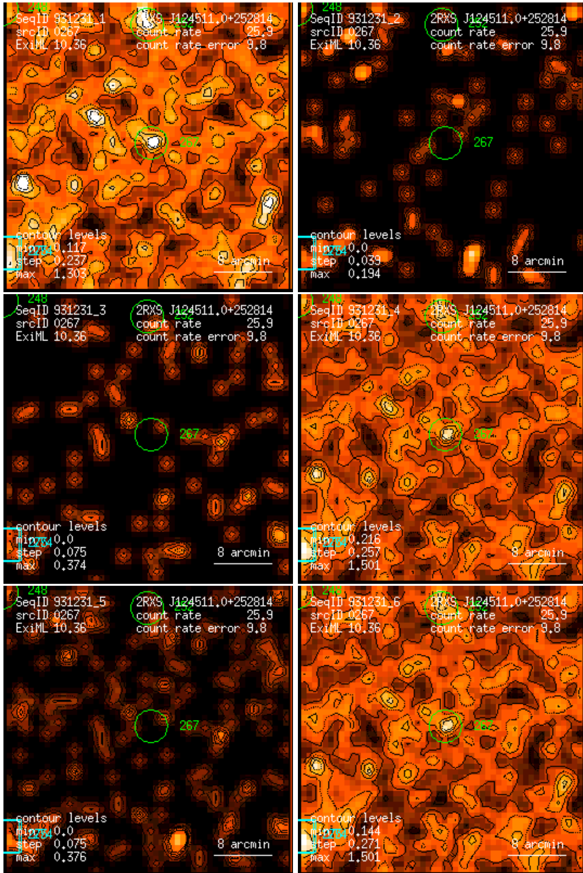
Figure 267: RASS 931231: detection 0267: band rate images, Gaussian filter: (1) PSPC channels 11 – 41, (2) 52 – 90, (3) 91 – 201, (4) 11 – 235, (5) 52 – 201, (6) 11 – 201. Broad band rates in counts/ks. Band rate contour levels in counts/ks/arcmin 2 .
